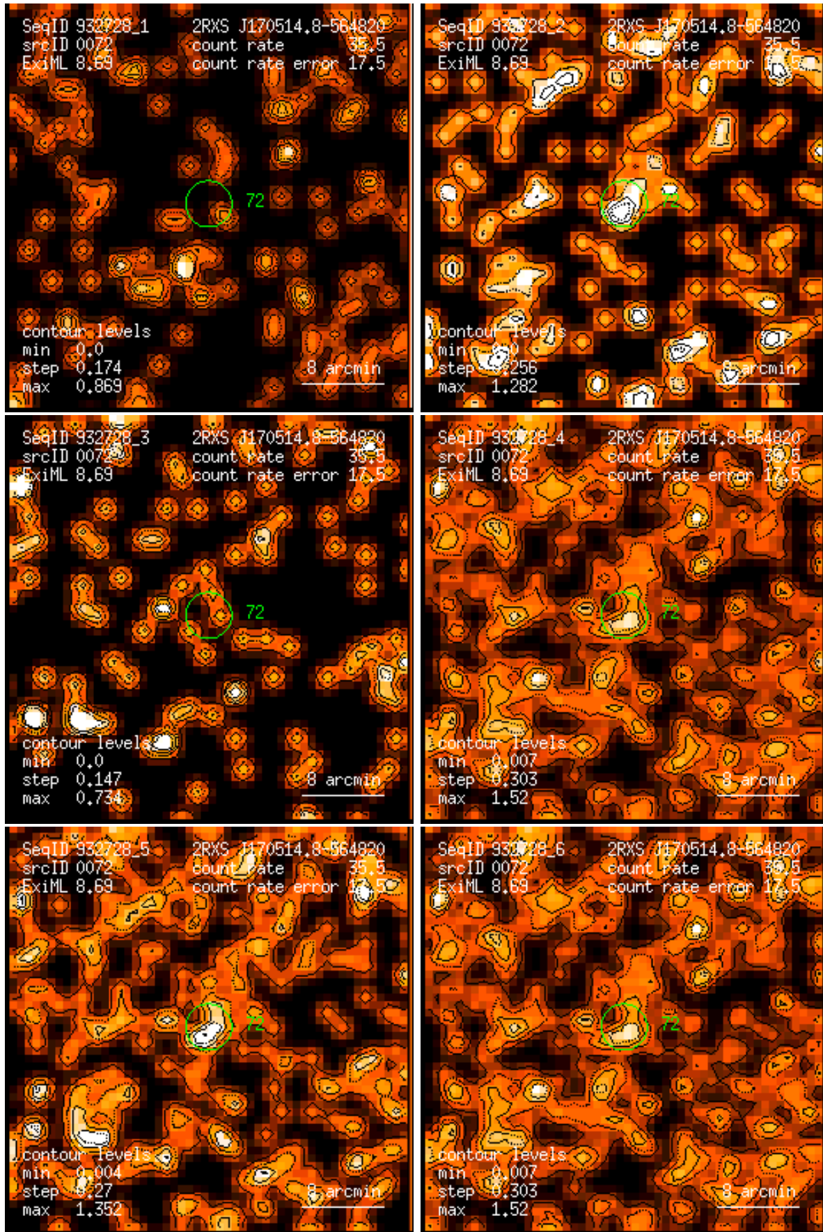
Figure 72: RASS 932728: detection 0072: band rate images, Gaussian filter: (1) PSPC channels 11 – 41, (2) 52 – 90, (3) 91 – 201, (4) 11 – 235, (5) 52 – 201, (6) 11 – 201. Broad band rates in counts/ks. Band rate contour levels in counts/ks/arcmin 2 .
