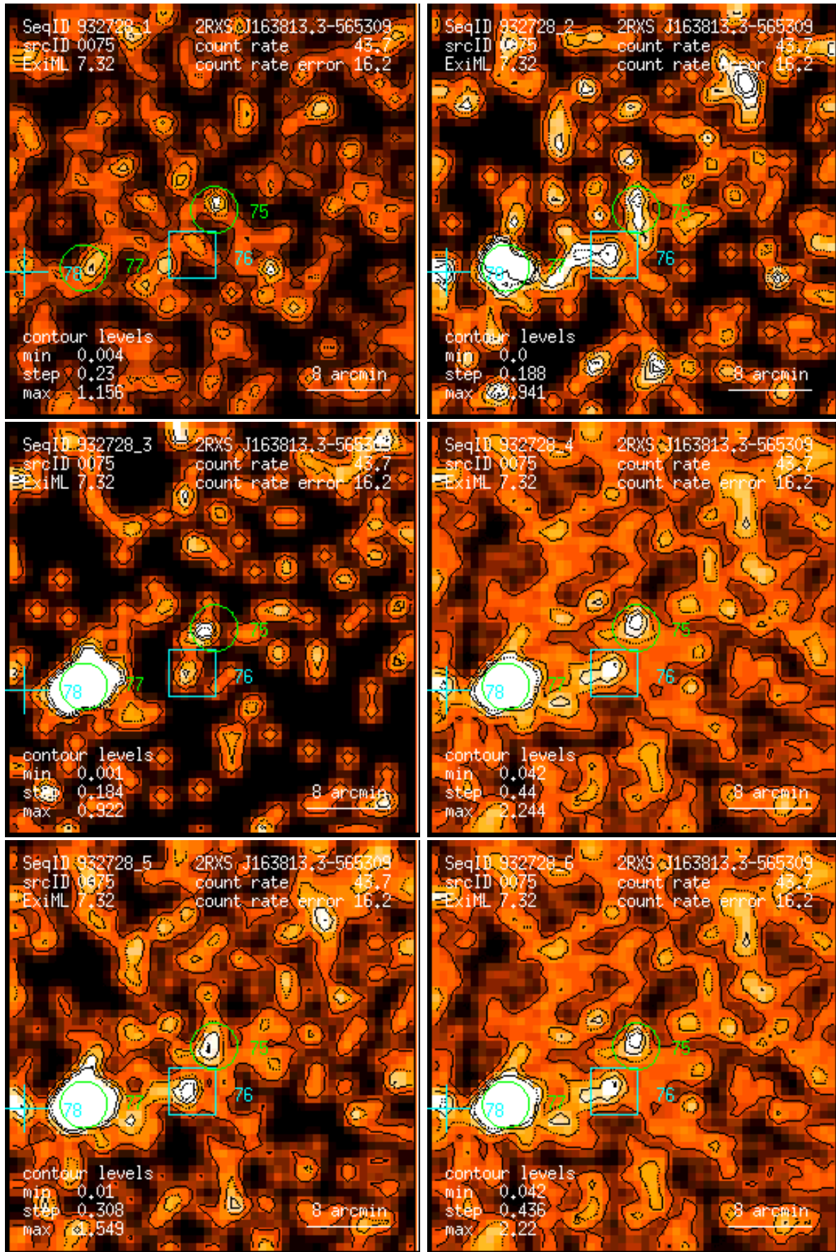
Figure 75: RASS 932728: detection 0075: band rate images, Gaussian filter: (1) PSPC channels 11 – 41, (2) 52 – 90, (3) 91 – 201, (4) 11 – 235, (5) 52 – 201, (6) 11 – 201. Broad band rates in counts/ks. Band rate contour levels in counts/ks/arcmin 2 .
