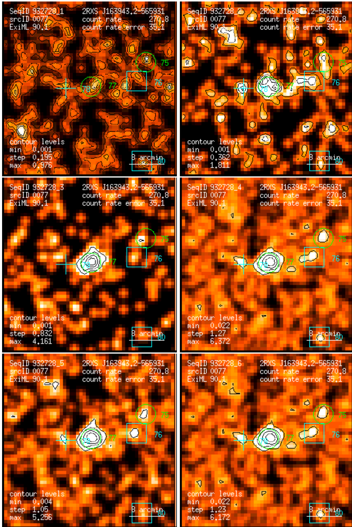
Figure 77: RASS 932728: detection 0077: band rate images, Gaussian filter: (1) PSPC channels 11 – 41, (2) 52 – 90, (3) 91 – 201, (4) 11 – 235, (5) 52 – 201, (6) 11 – 201. Broad band rates in counts/ks. Band rate contour levels in counts/ks/arcmin 2 .
