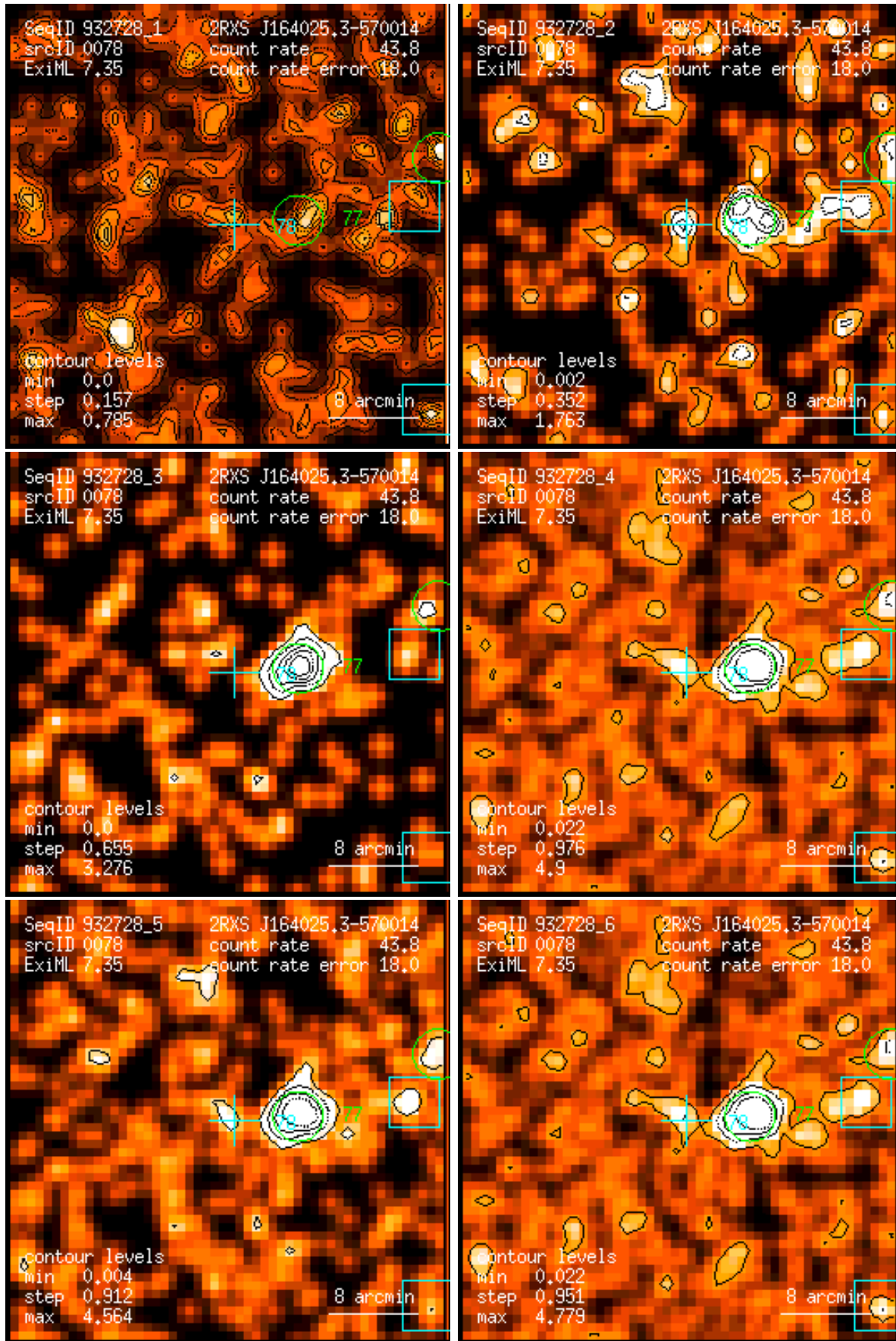
Figure 78: RASS 932728: detection 0078: band rate images, Gaussian filter: (1) PSPC channels 11 – 41, (2) 52 – 90, (3) 91 – 201, (4) 11 – 235, (5) 52 – 201, (6) 11 – 201. Broad band rates in counts/ks. Band rate contour levels in counts/ks/arcmin 2 .
