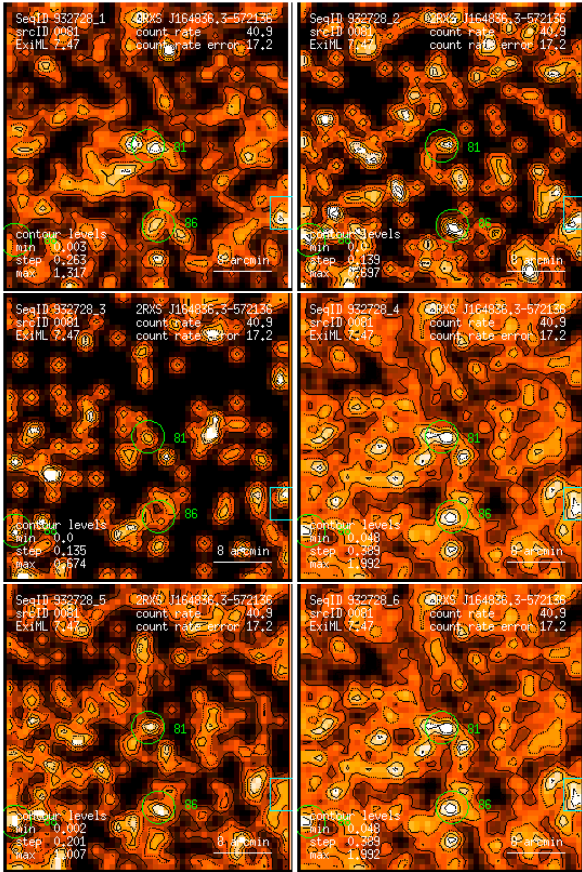
Figure 81: RASS 932728: detection 0081: band rate images, Gaussian filter: (1) PSPC channels 11 – 41, (2) 52 – 90, (3) 91 – 201, (4) 11 – 235, (5) 52 – 201, (6) 11 – 201. Broad band rates in counts/ks. Band rate contour levels in counts/ks/arcmin 2 .
