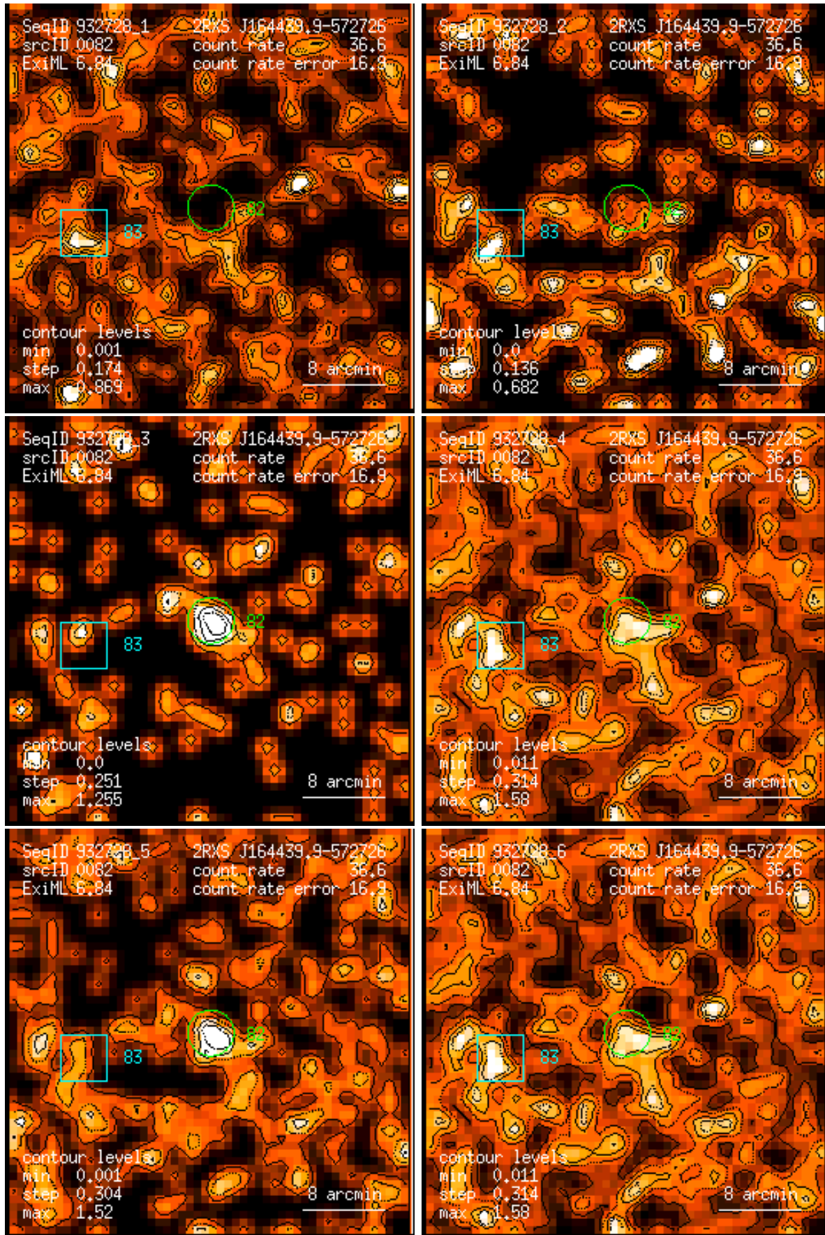
Figure 82: RASS 932728: detection 0082: band rate images, Gaussian filter: (1) PSPC channels 11 – 41, (2) 52 – 90, (3) 91 – 201, (4) 11 – 235, (5) 52 – 201, (6) 11 – 201. Broad band rates in counts/ks. Band rate contour levels in counts/ks/arcmin 2 .
