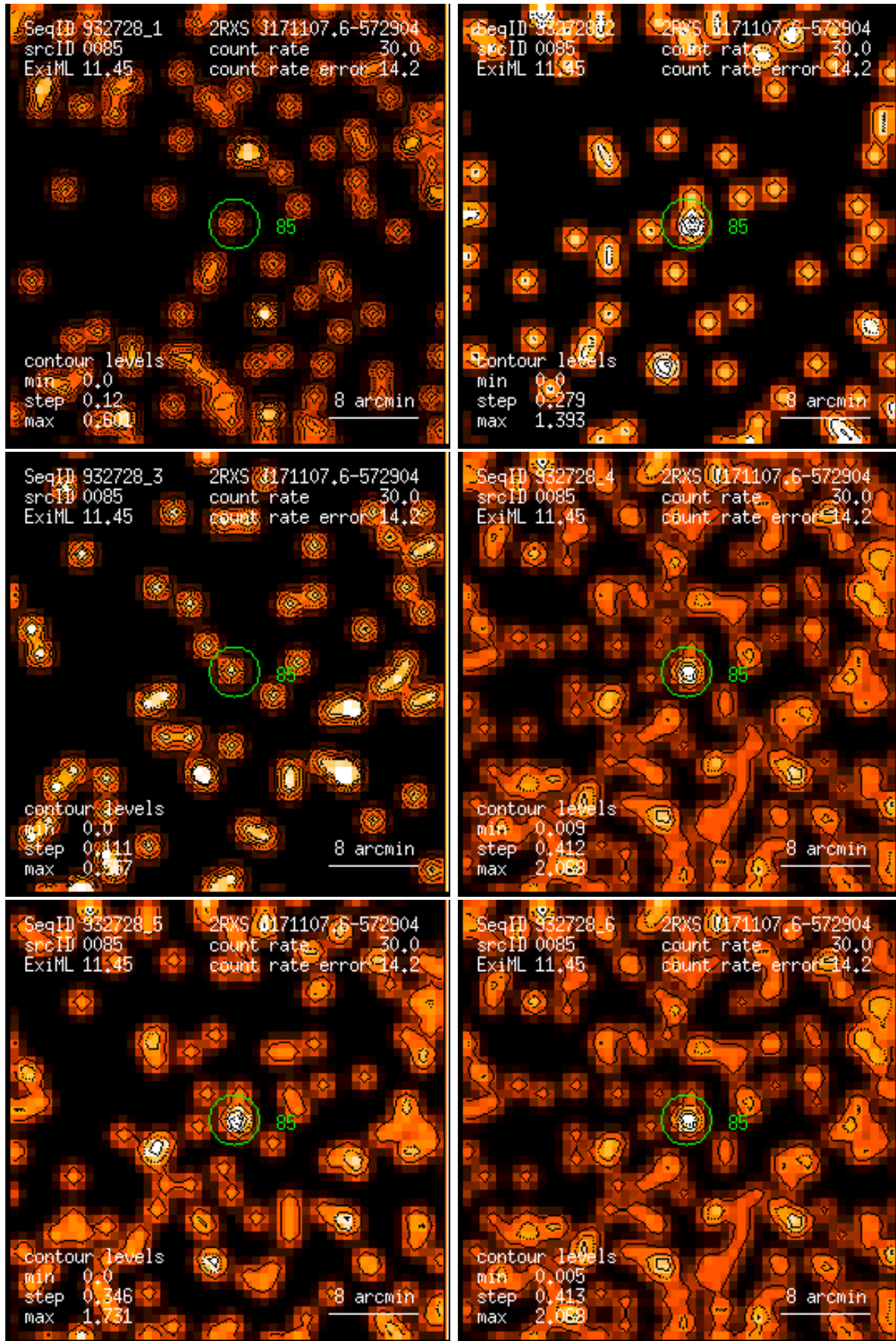
Figure 85: RASS 932728: detection 0085: band rate images, Gaussian filter: (1) PSPC channels 11 – 41, (2) 52 – 90, (3) 91 – 201, (4) 11 – 235, (5) 52 – 201, (6) 11 – 201. Broad band rates in counts/ks. Band rate contour levels in counts/ks/arcmin 2 .
