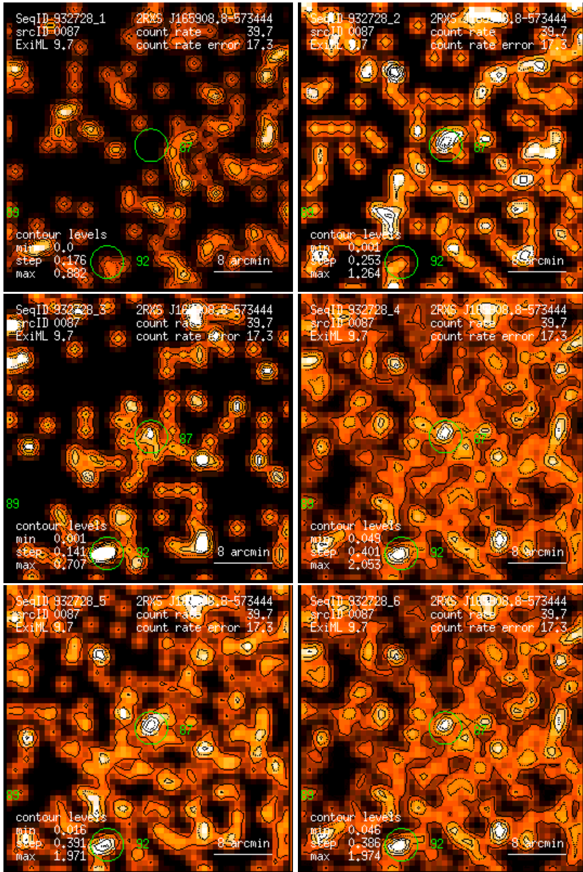
Figure 87: RASS 932728: detection 0087: band rate images, Gaussian filter: (1) PSPC channels 11 – 41, (2) 52 – 90, (3) 91 – 201, (4) 11 – 235, (5) 52 – 201, (6) 11 – 201. Broad band rates in counts/ks. Band rate contour levels in counts/ks/arcmin 2 .
