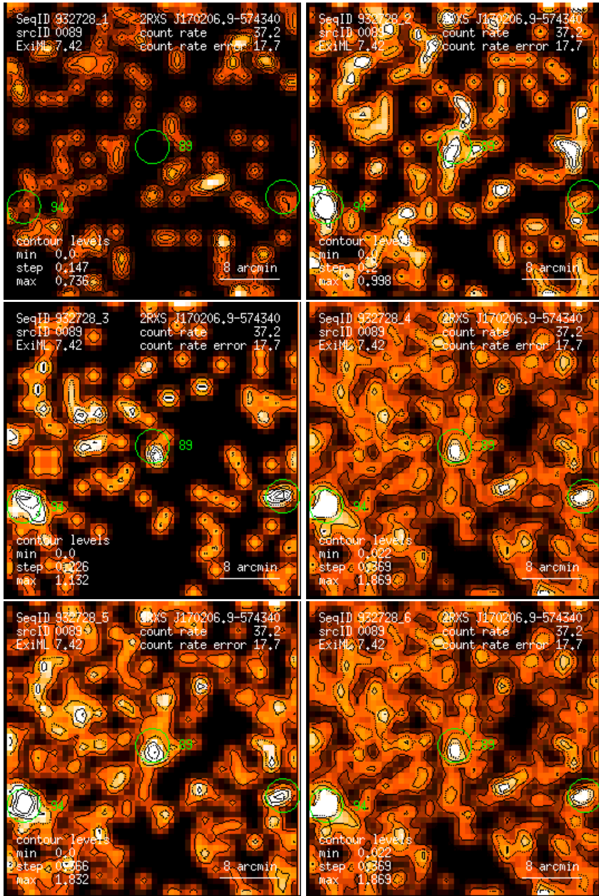
Figure 89: RASS 932728: detection 0089: band rate images, Gaussian filter: (1) PSPC channels 11 – 41, (2) 52 – 90, (3) 91 – 201, (4) 11 – 235, (5) 52 – 201, (6) 11 – 201. Broad band rates in counts/ks. Band rate contour levels in counts/ks/arcmin 2 .
