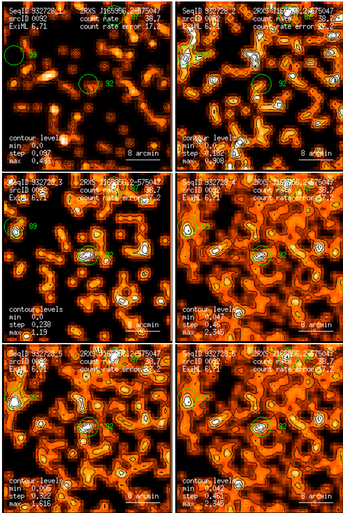
Figure 92: RASS 932728: detection 0092: band rate images, Gaussian filter: (1) PSPC channels 11 – 41, (2) 52 – 90, (3) 91 – 201, (4) 11 – 235, (5) 52 – 201, (6) 11 – 201. Broad band rates in counts/ks. Band rate contour levels in counts/ks/arcmin 2 .
