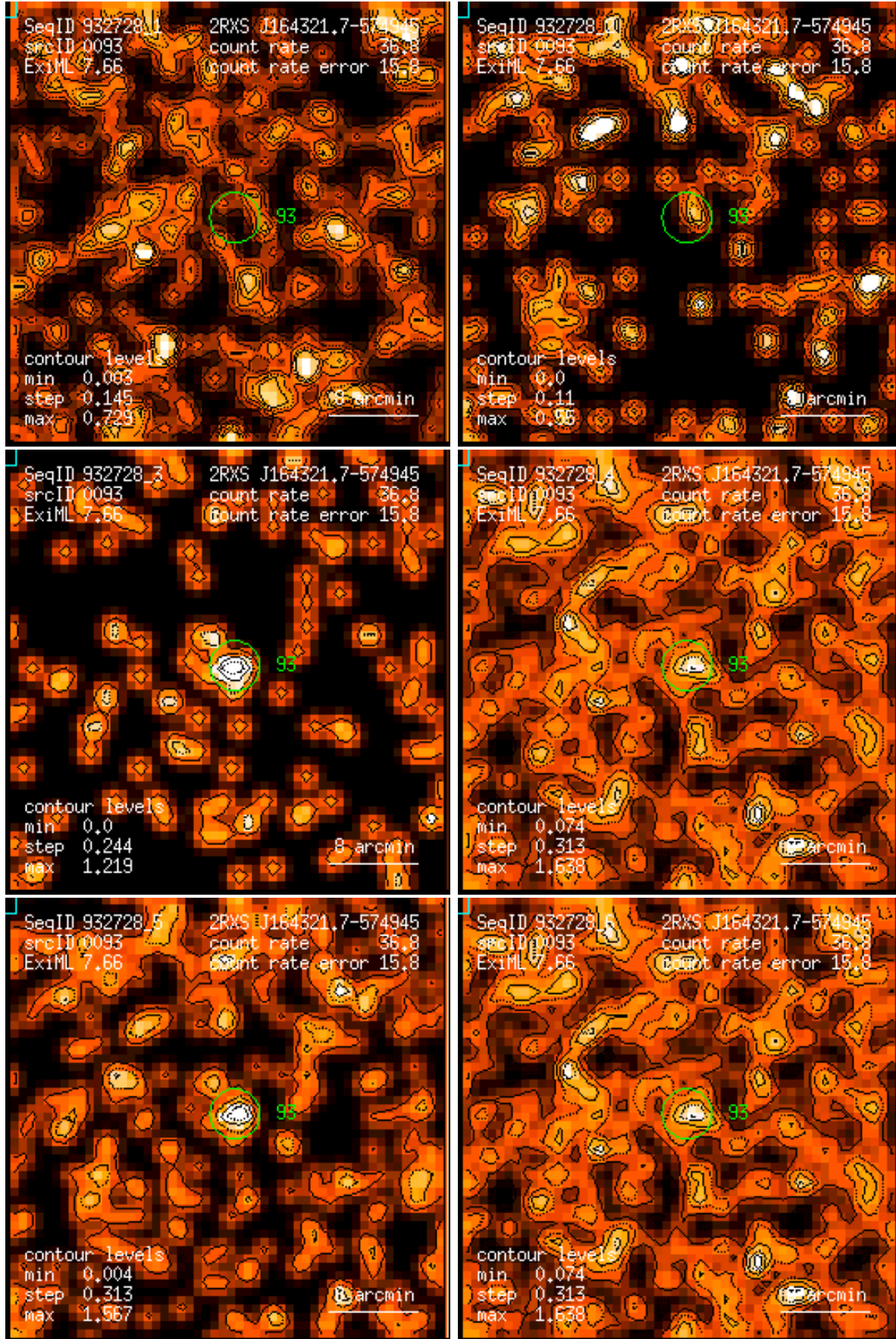
Figure 93: RASS 932728: detection 0093: band rate images, Gaussian filter: (1) PSPC channels 11 – 41, (2) 52 – 90, (3) 91 – 201, (4) 11 – 235, (5) 52 – 201, (6) 11 – 201. Broad band rates in counts/ks. Band rate contour levels in counts/ks/arcmin 2 .
