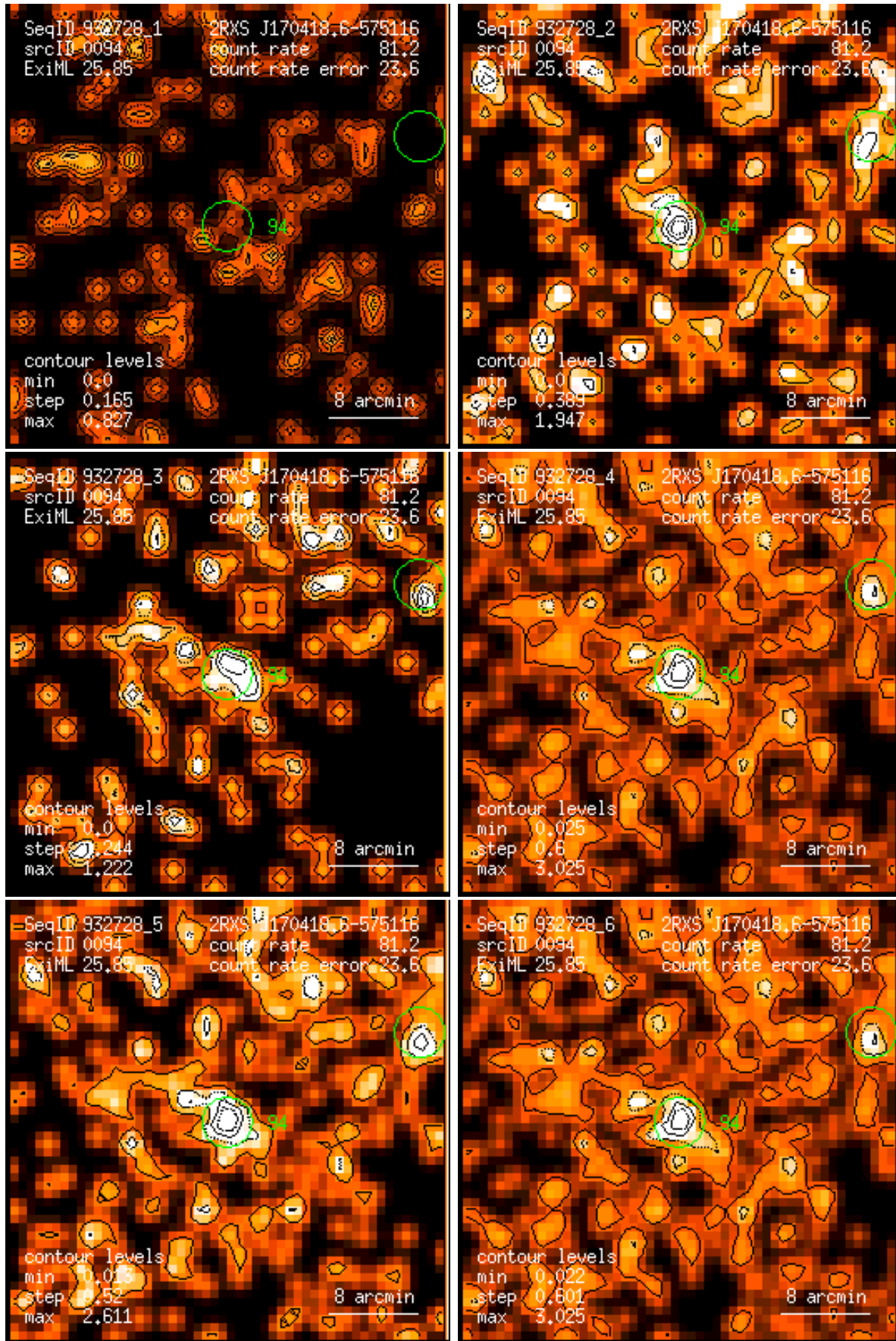
Figure 94: RASS 932728: detection 0094: band rate images, Gaussian filter: (1) PSPC channels 11 – 41, (2) 52 – 90, (3) 91 – 201, (4) 11 – 235, (5) 52 – 201, (6) 11 – 201. Broad band rates in counts/ks. Band rate contour levels in counts/ks/arcmin 2 .
