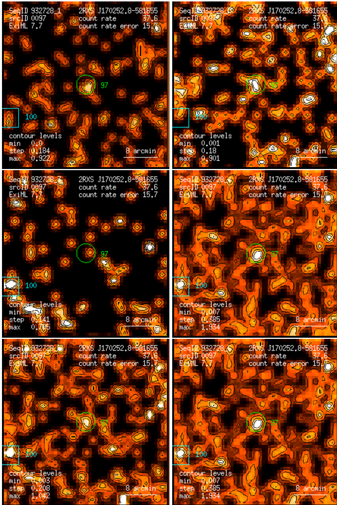
Figure 97: RASS 932728: detection 0097: band rate images, Gaussian filter: (1) PSPC channels 11 – 41, (2) 52 – 90, (3) 91 – 201, (4) 11 – 235, (5) 52 – 201, (6) 11 – 201. Broad band rates in counts/ks. Band rate contour levels in counts/ks/arcmin 2 .
