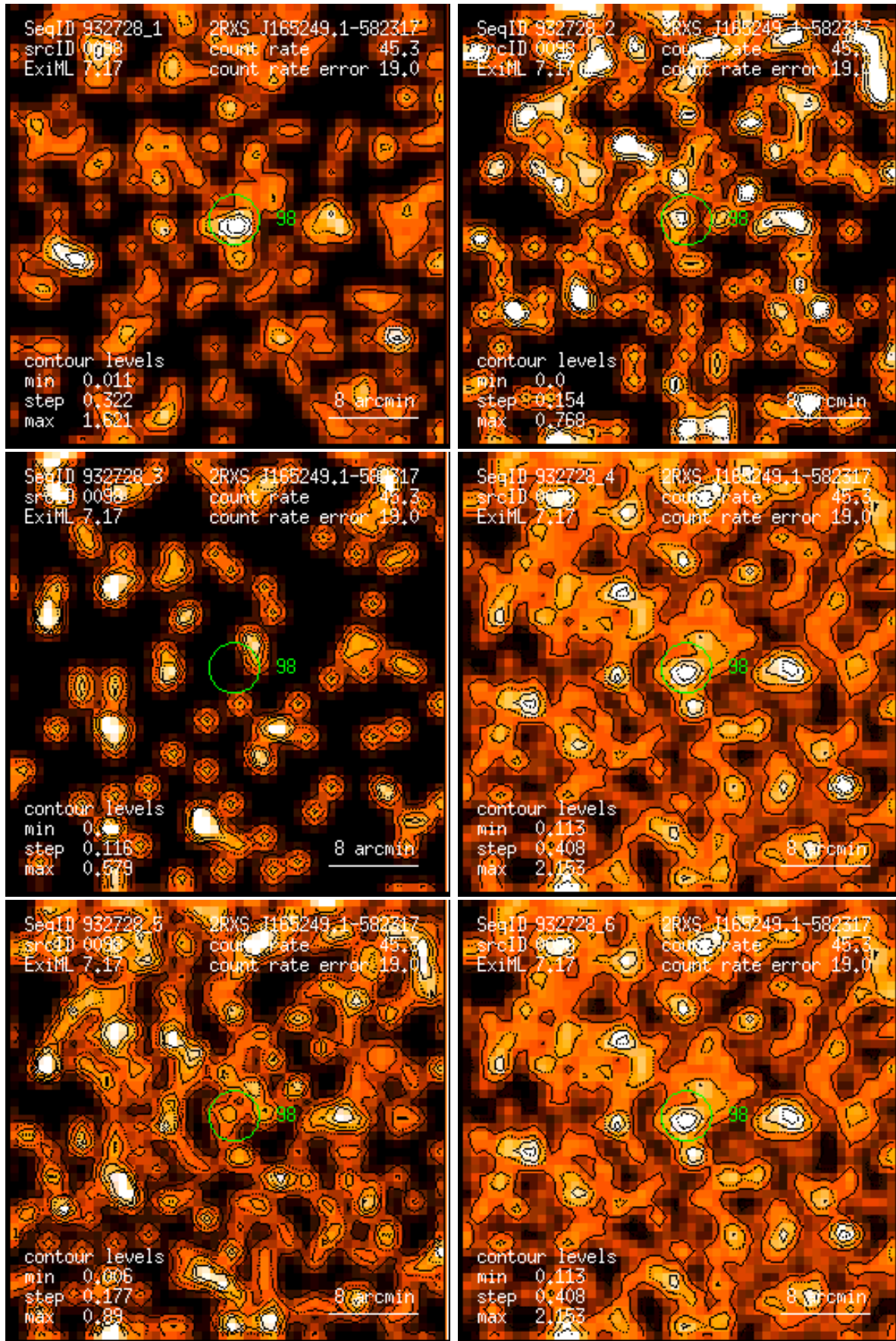
Figure 98: RASS 932728: detection 0098: band rate images, Gaussian filter: (1) PSPC channels 11 – 41, (2) 52 – 90, (3) 91 – 201, (4) 11 – 235, (5) 52 – 201, (6) 11 – 201. Broad band rates in counts/ks. Band rate contour levels in counts/ks/arcmin 2 .
