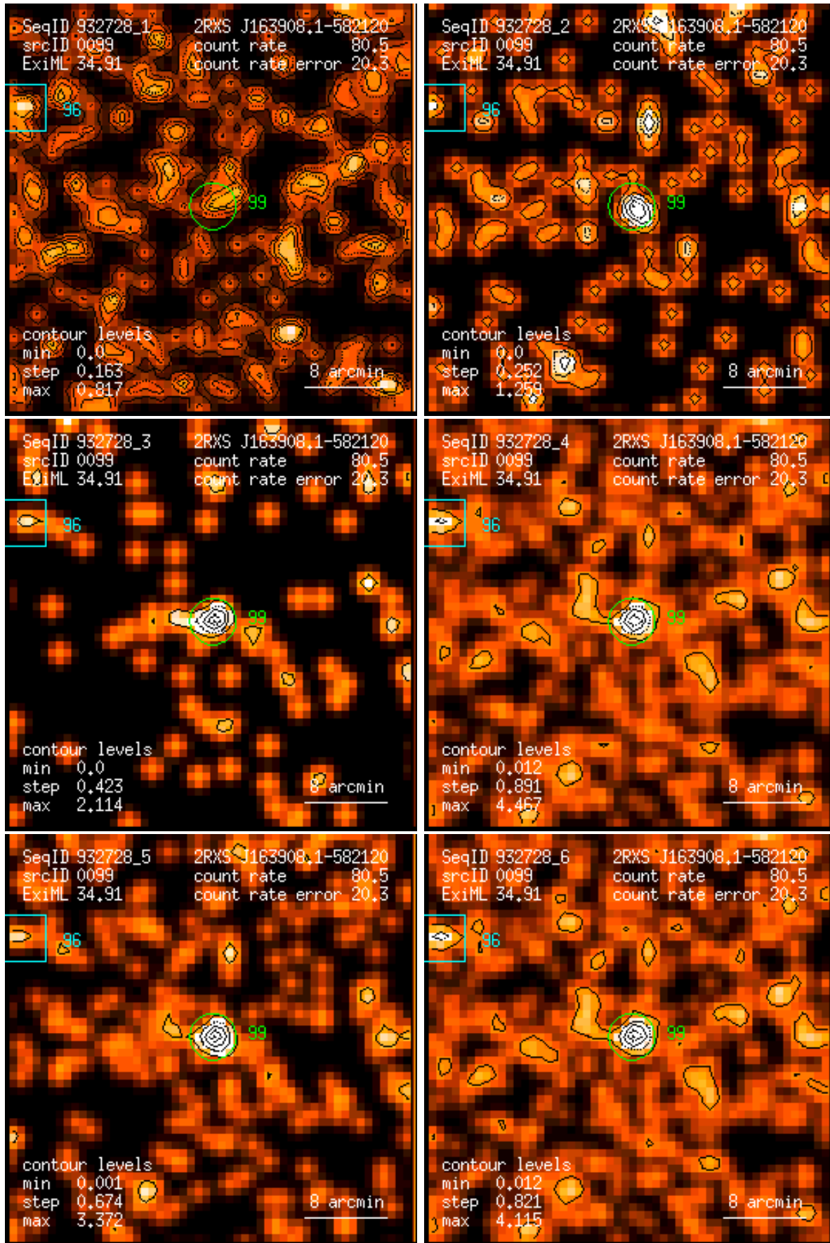
Figure 99: RASS 932728: detection 0099: band rate images, Gaussian filter: (1) PSPC channels 11 – 41, (2) 52 – 90, (3) 91 – 201, (4) 11 – 235, (5) 52 – 201, (6) 11 – 201. Broad band rates in counts/ks. Band rate contour levels in counts/ks/arcmin 2 .
