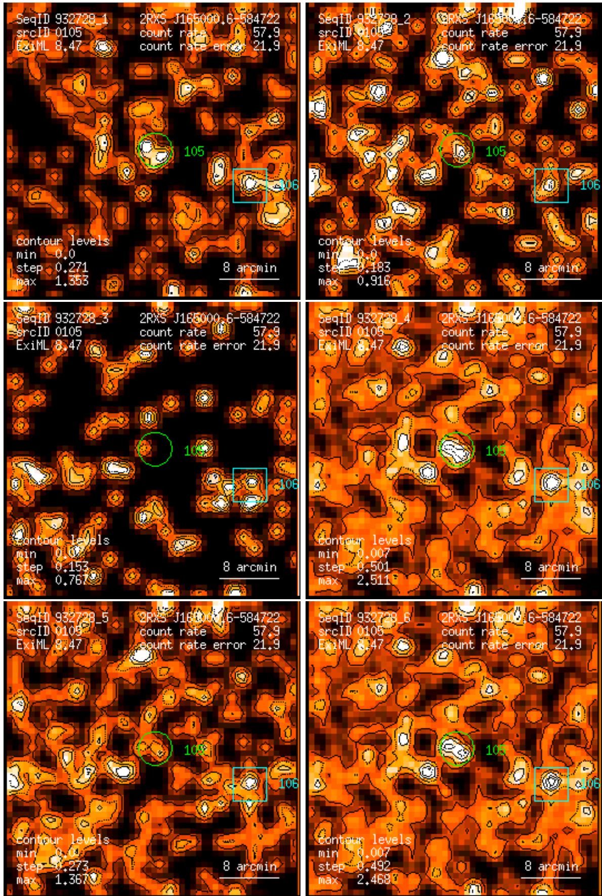
Figure 105: RASS 932728: detection 0105: band rate images, Gaussian filter: (1) PSPC channels 11 – 41, (2) 52 – 90, (3) 91 – 201, (4) 11 – 235, (5) 52 – 201, (6) 11 – 201. Broad band rates in counts/ks. Band rate contour levels in counts/ks/arcmin 2 .
