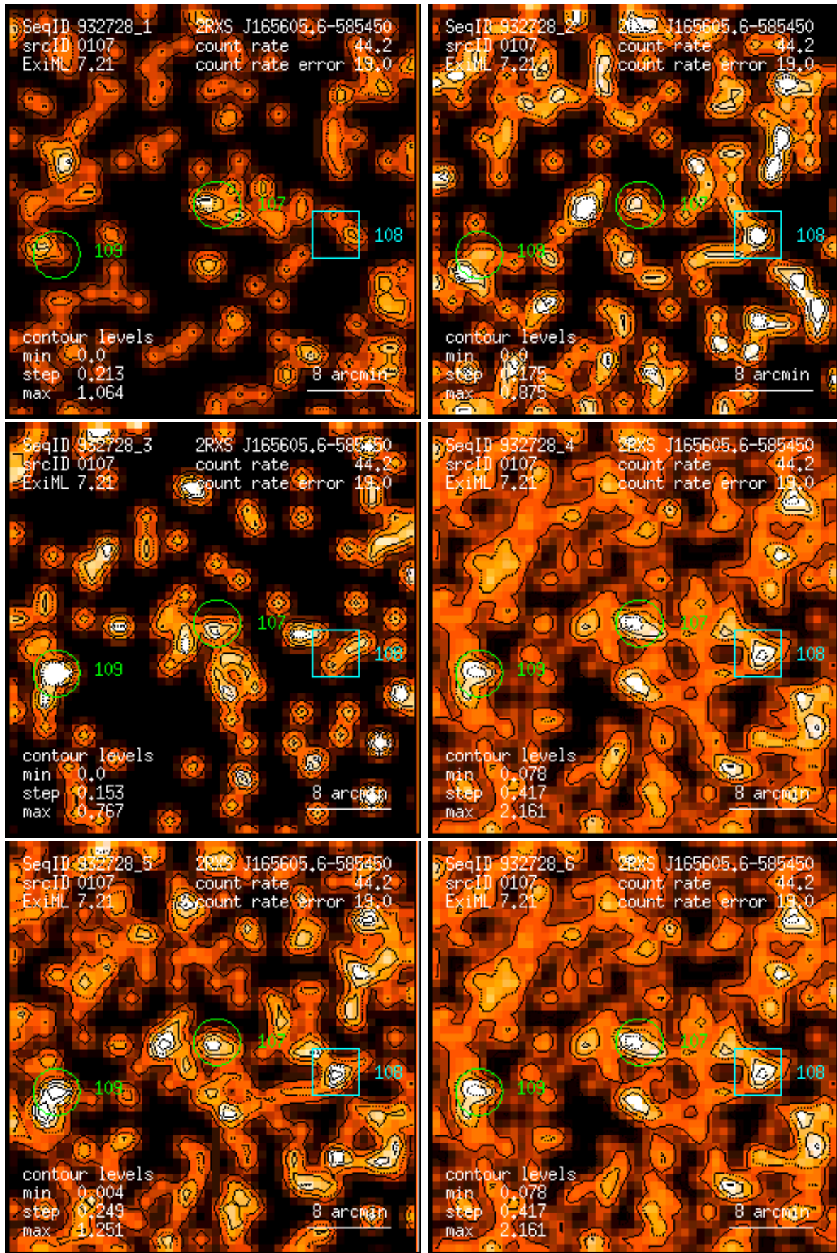
Figure 107: RASS 932728: detection 0107: band rate images, Gaussian filter: (1) PSPC channels 11 – 41, (2) 52 – 90, (3) 91 – 201, (4) 11 – 235, (5) 52 – 201, (6) 11 – 201. Broad band rates in counts/ks. Band rate contour levels in counts/ks/arcmin 2 .
