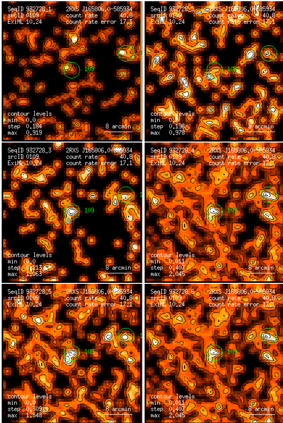
Figure 109: RASS 932728: detection 0109: band rate images, Gaussian filter: (1) PSPC channels 11 – 41, (2) 52 – 90, (3) 91 – 201, (4) 11 – 235, (5) 52 – 201, (6) 11 – 201. Broad band rates in counts/ks. Band rate contour levels in counts/ks/arcmin 2 .
