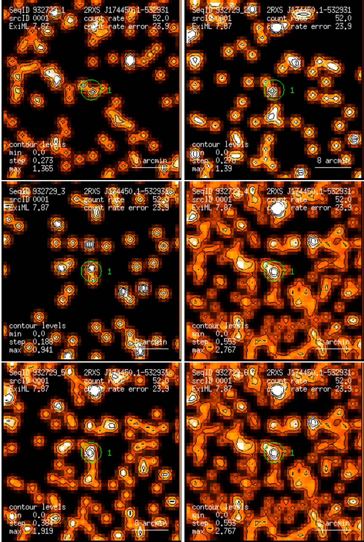
Figure 1: RASS 932729: detection 0001: band rate images, Gaussian filter: (1) PSPC channels 11 – 41, (2) 52 – 90, (3) 91 – 201, (4) 11 – 235, (5) 52 – 201, (6) 11 – 201. Broad band rates in counts/ks. Band rate contour levels in counts/ks/arcmin 2 .
