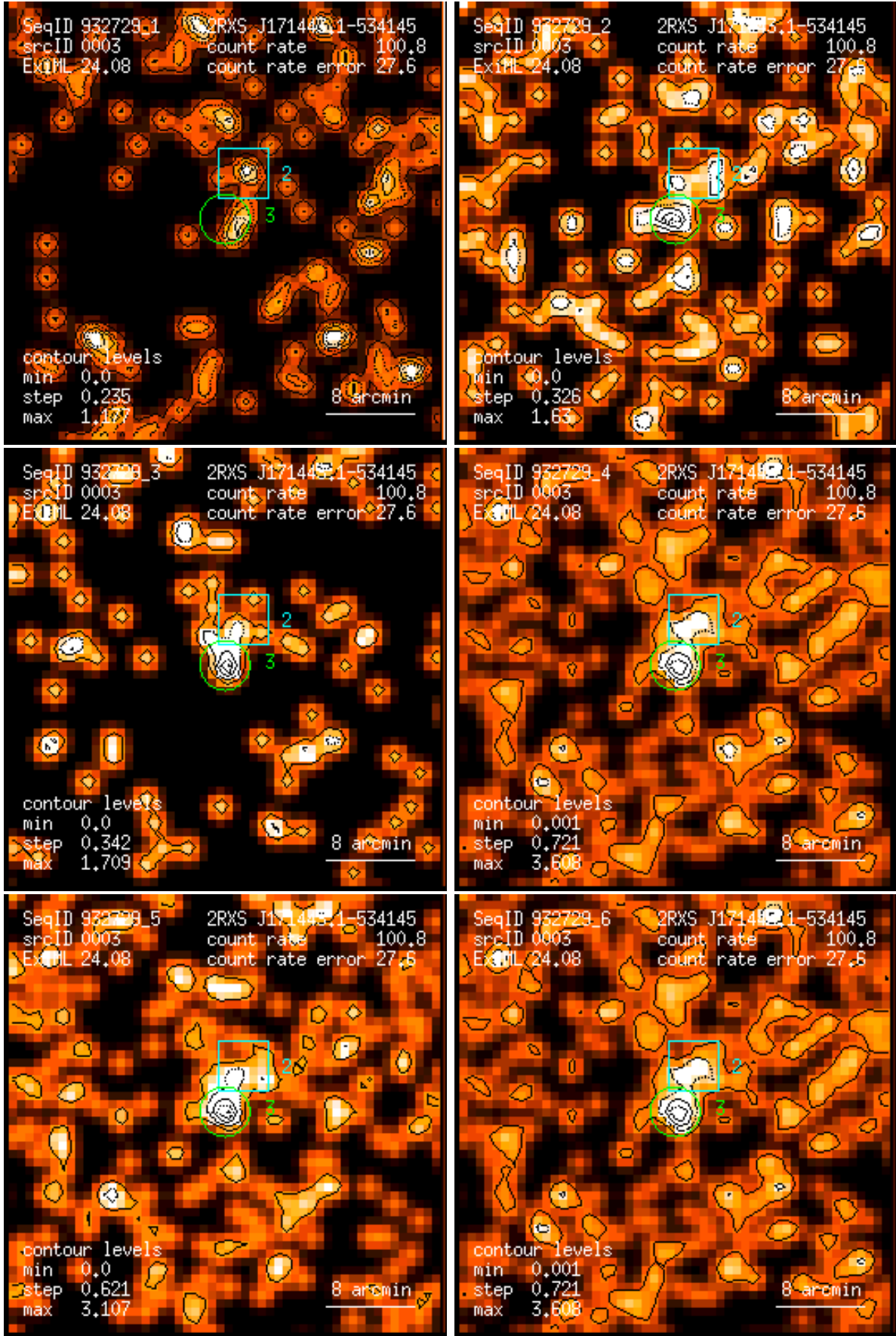
Figure 3: RASS 932729: detection 0003: band rate images, Gaussian filter: (1) PSPC channels 11 – 41, (2) 52 – 90, (3) 91 – 201, (4) 11 – 235, (5) 52 – 201, (6) 11 – 201. Broad band rates in counts/ks. Band rate contour levels in counts/ks/arcmin 2 .
