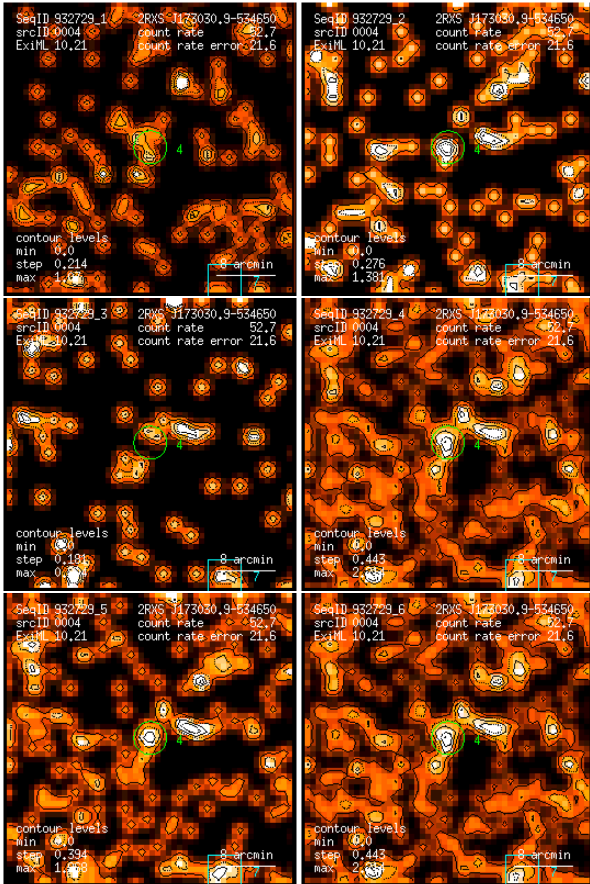
Figure 4: RASS 932729: detection 0004: band rate images, Gaussian filter: (1) PSPC channels 11 – 41, (2) 52 – 90, (3) 91 – 201, (4) 11 – 235, (5) 52 – 201, (6) 11 – 201. Broad band rates in counts/ks. Band rate contour levels in counts/ks/arcmin 2 .
