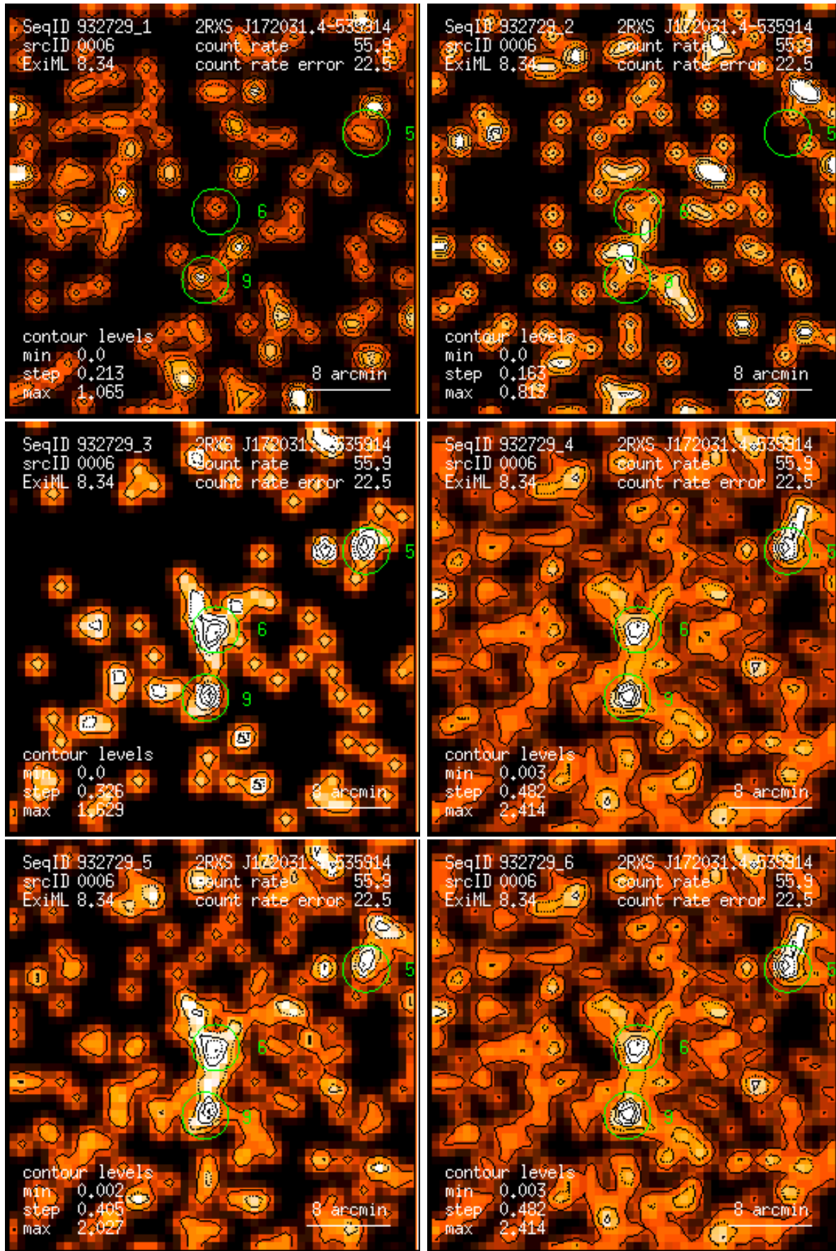
Figure 6: RASS 932729: detection 0006: band rate images, Gaussian filter: (1) PSPC channels 11 – 41, (2) 52 – 90, (3) 91 – 201, (4) 11 – 235, (5) 52 – 201, (6) 11 – 201. Broad band rates in counts/ks. Band rate contour levels in counts/ks/arcmin 2 .
