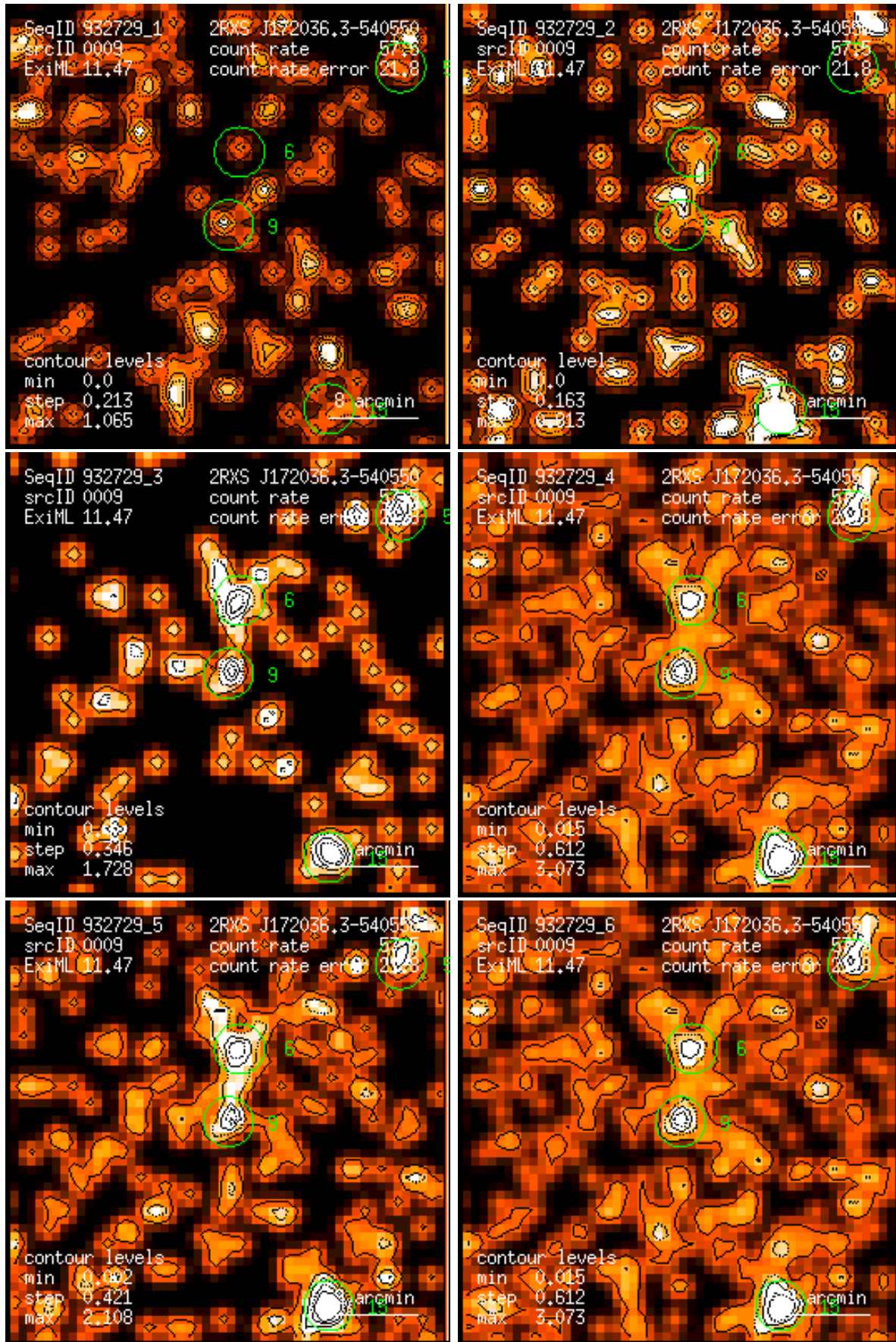
Figure 9: RASS 932729: detection 0009: band rate images, Gaussian filter: (1) PSPC channels 11 – 41, (2) 52 – 90, (3) 91 – 201, (4) 11 – 235, (5) 52 – 201, (6) 11 – 201. Broad band rates in counts/ks. Band rate contour levels in counts/ks/arcmin 2 .
