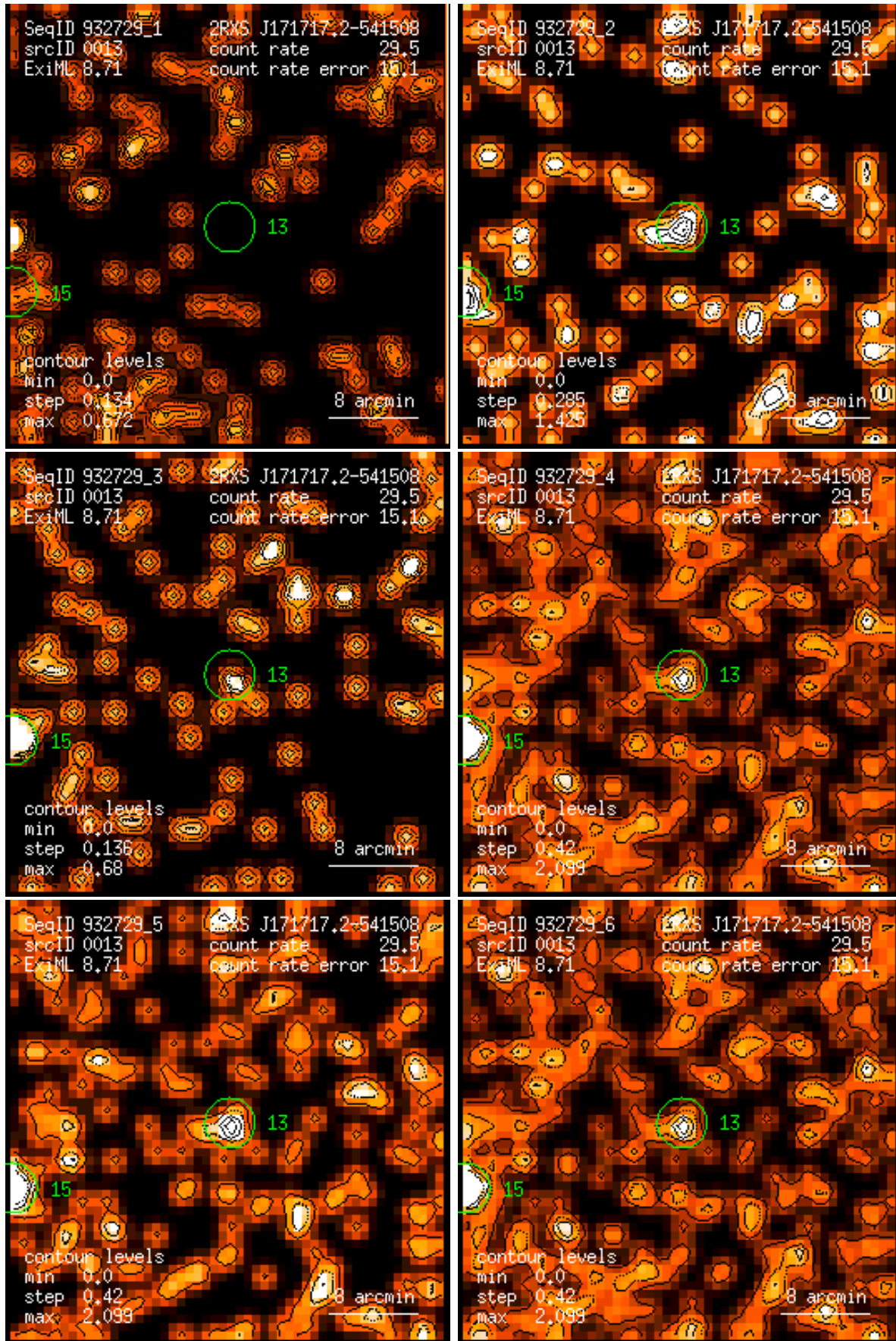
Figure 13: RASS 932729: detection 0013: band rate images, Gaussian filter: (1) PSPC channels 11 – 41, (2) 52 – 90, (3) 91 – 201, (4) 11 – 235, (5) 52 – 201, (6) 11 – 201. Broad band rates in counts/ks. Band rate contour levels in counts/ks/arcmin 2 .
