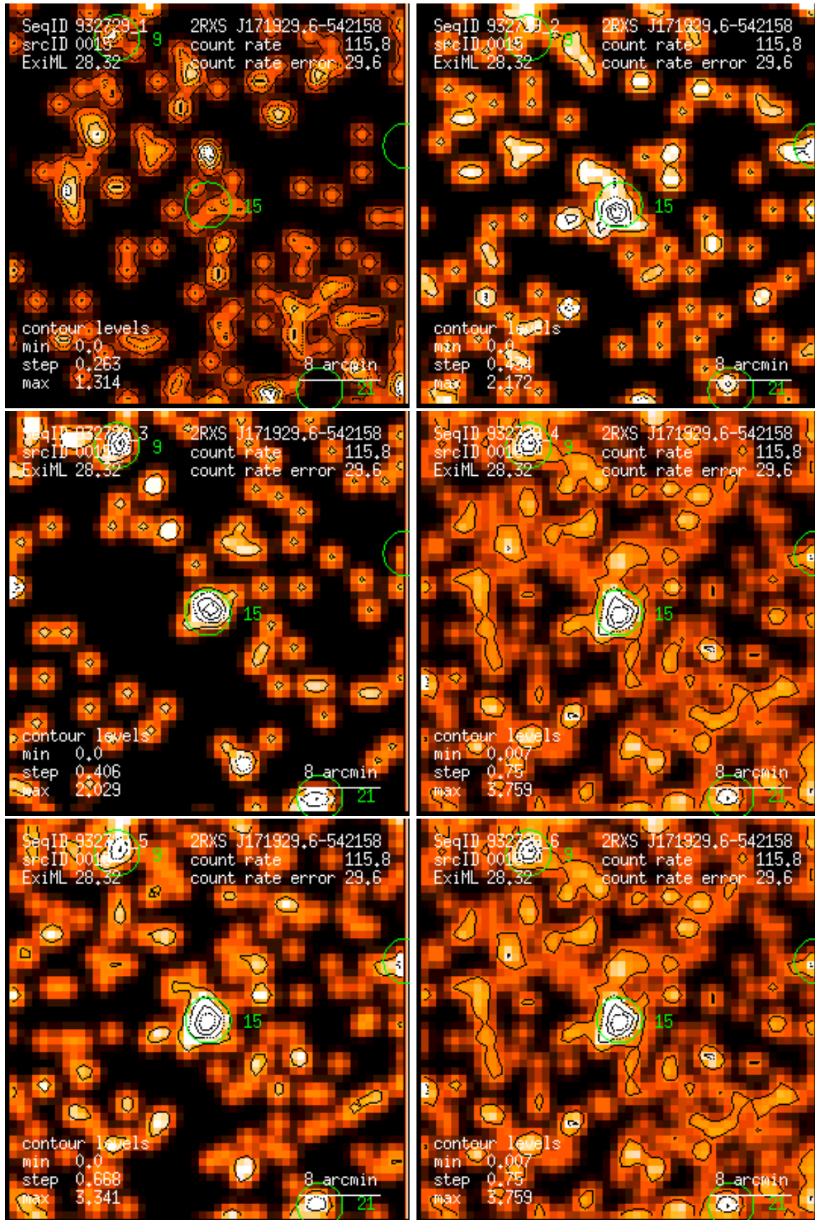
Figure 15: RASS 932729: detection 0015: band rate images, Gaussian filter: (1) PSPC channels 11 – 41, (2) 52 – 90, (3) 91 – 201, (4) 11 – 235, (5) 52 – 201, (6) 11 – 201. Broad band rates in counts/ks. Band rate contour levels in counts/ks/arcmin 2 .
