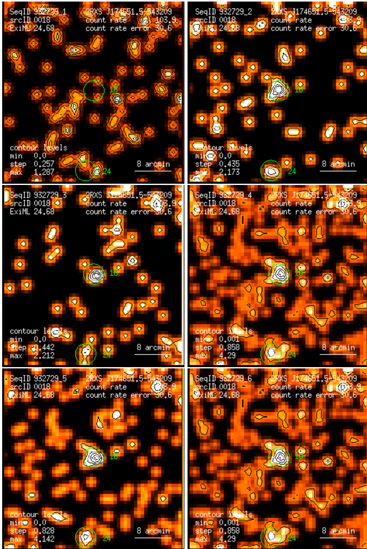
Figure 18: RASS 932729: detection 0018: band rate images, Gaussian filter: (1) PSPC channels 11 – 41, (2) 52 – 90, (3) 91 – 201, (4) 11 – 235, (5) 52 – 201, (6) 11 – 201. Broad band rates in counts/ks. Band rate contour levels in counts/ks/arcmin 2 .
