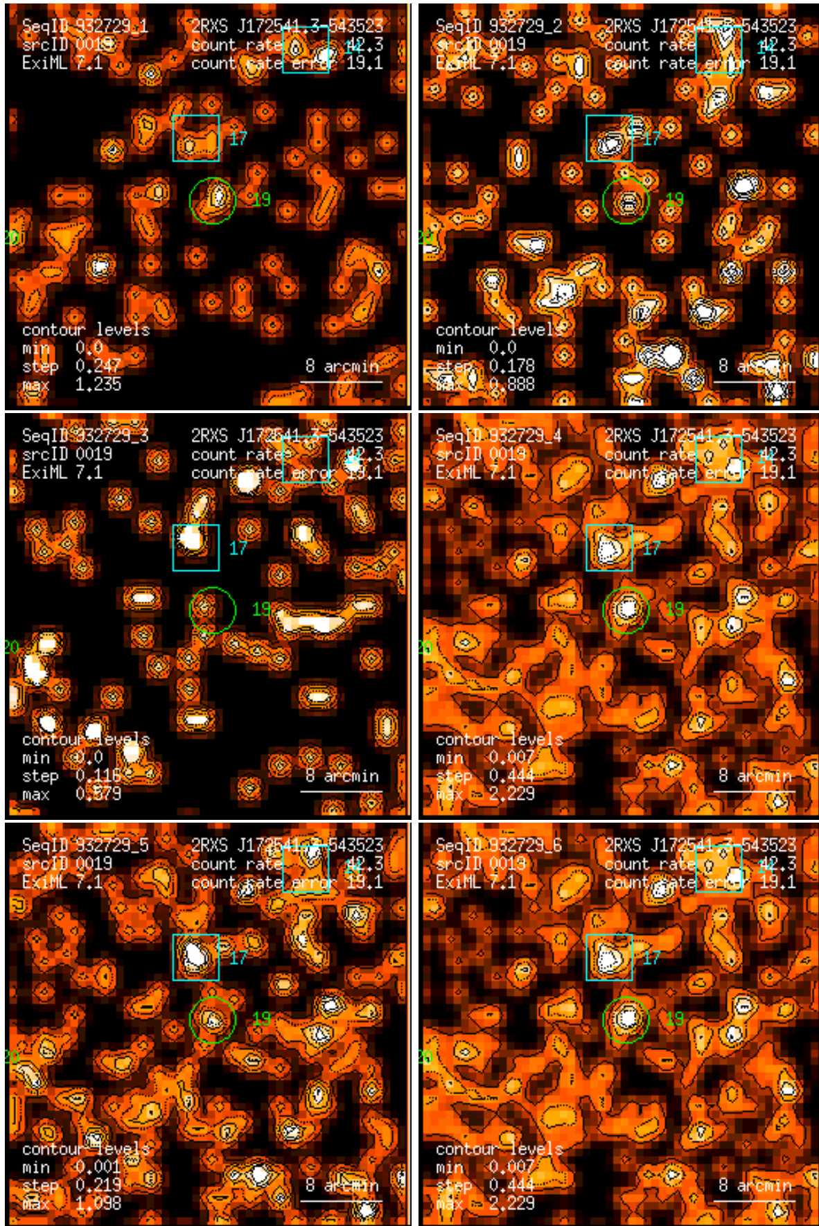
Figure 19: RASS 932729: detection 0019: band rate images, Gaussian filter: (1) PSPC channels 11 – 41, (2) 52 – 90, (3) 91 – 201, (4) 11 – 235, (5) 52 – 201, (6) 11 – 201. Broad band rates in counts/ks. Band rate contour levels in counts/ks/arcmin 2 .
