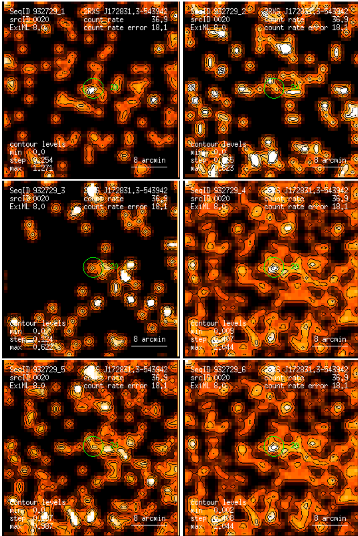
Figure 20: RASS 932729: detection 0020: band rate images, Gaussian filter: (1) PSPC channels 11 – 41, (2) 52 – 90, (3) 91 – 201, (4) 11 – 235, (5) 52 – 201, (6) 11 – 201. Broad band rates in counts/ks. Band rate contour levels in counts/ks/arcmin 2 .
