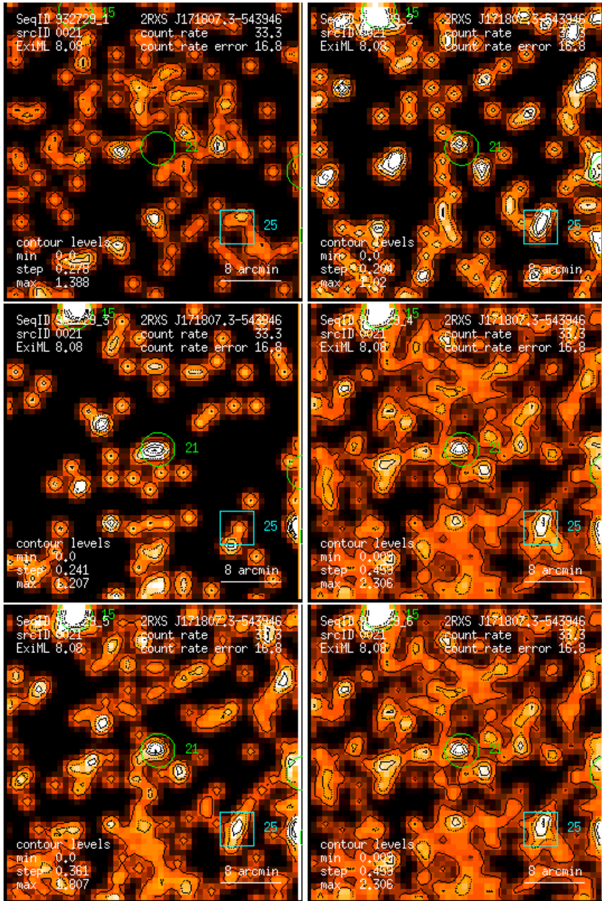
Figure 21: RASS 932729: detection 0021: band rate images, Gaussian filter: (1) PSPC channels 11 – 41, (2) 52 – 90, (3) 91 – 201, (4) 11 – 235, (5) 52 – 201, (6) 11 – 201. Broad band rates in counts/ks. Band rate contour levels in counts/ks/arcmin 2 .
