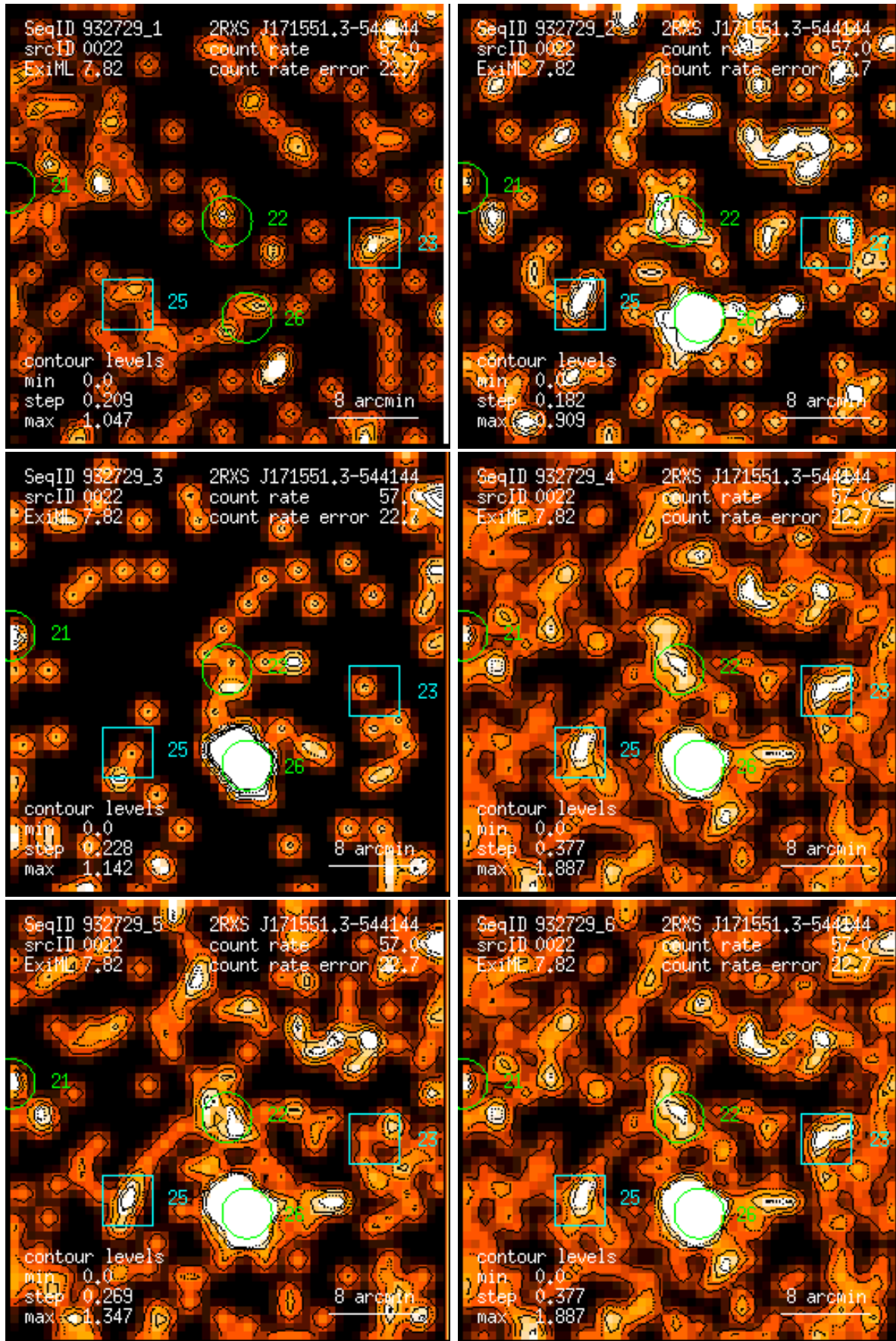
Figure 22: RASS 932729: detection 0022: band rate images, Gaussian filter: (1) PSPC channels 11 – 41, (2) 52 – 90, (3) 91 – 201, (4) 11 – 235, (5) 52 – 201, (6) 11 – 201. Broad band rates in counts/ks. Band rate contour levels in counts/ks/arcmin 2 .
