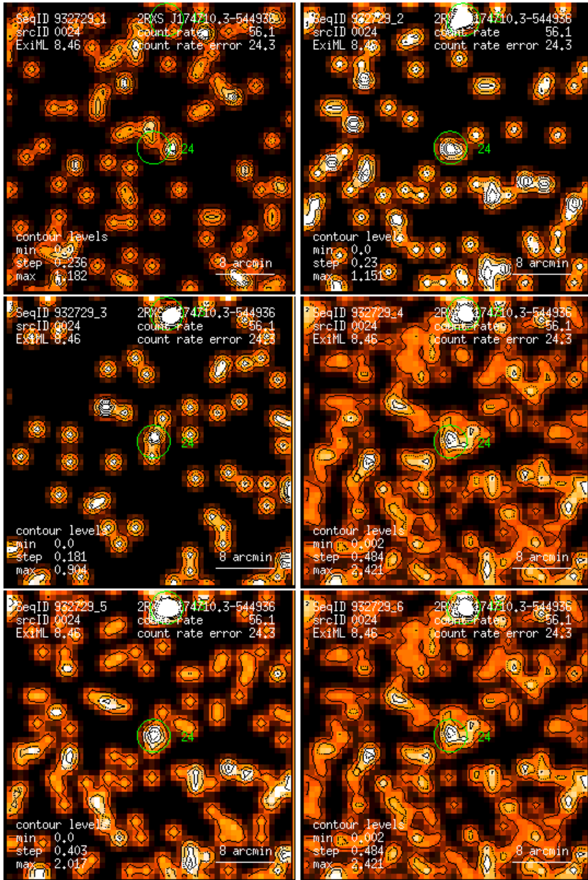
Figure 24: RASS 932729: detection 0024: band rate images, Gaussian filter: (1) PSPC channels 11 – 41, (2) 52 – 90, (3) 91 – 201, (4) 11 – 235, (5) 52 – 201, (6) 11 – 201. Broad band rates in counts/ks. Band rate contour levels in counts/ks/arcmin 2 .
