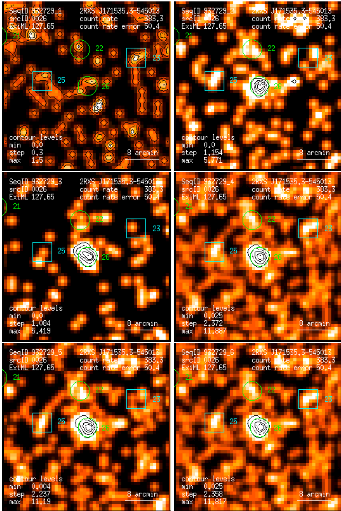
Figure 26: RASS 932729: detection 0026: band rate images, Gaussian filter: (1) PSPC channels 11 – 41, (2) 52 – 90, (3) 91 – 201, (4) 11 – 235, (5) 52 – 201, (6) 11 – 201. Broad band rates in counts/ks. Band rate contour levels in counts/ks/arcmin 2 .
