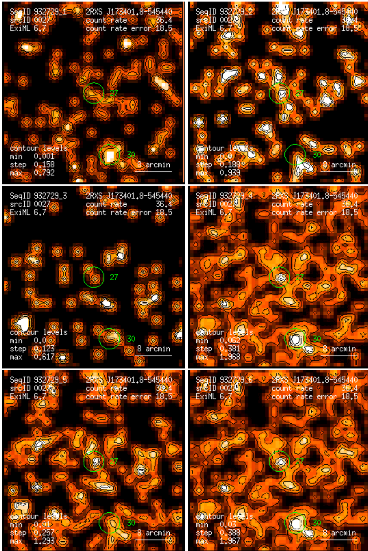
Figure 27: RASS 932729: detection 0027: band rate images, Gaussian filter: (1) PSPC channels 11 – 41, (2) 52 – 90, (3) 91 – 201, (4) 11 – 235, (5) 52 – 201, (6) 11 – 201. Broad band rates in counts/ks. Band rate contour levels in counts/ks/arcmin 2 .
