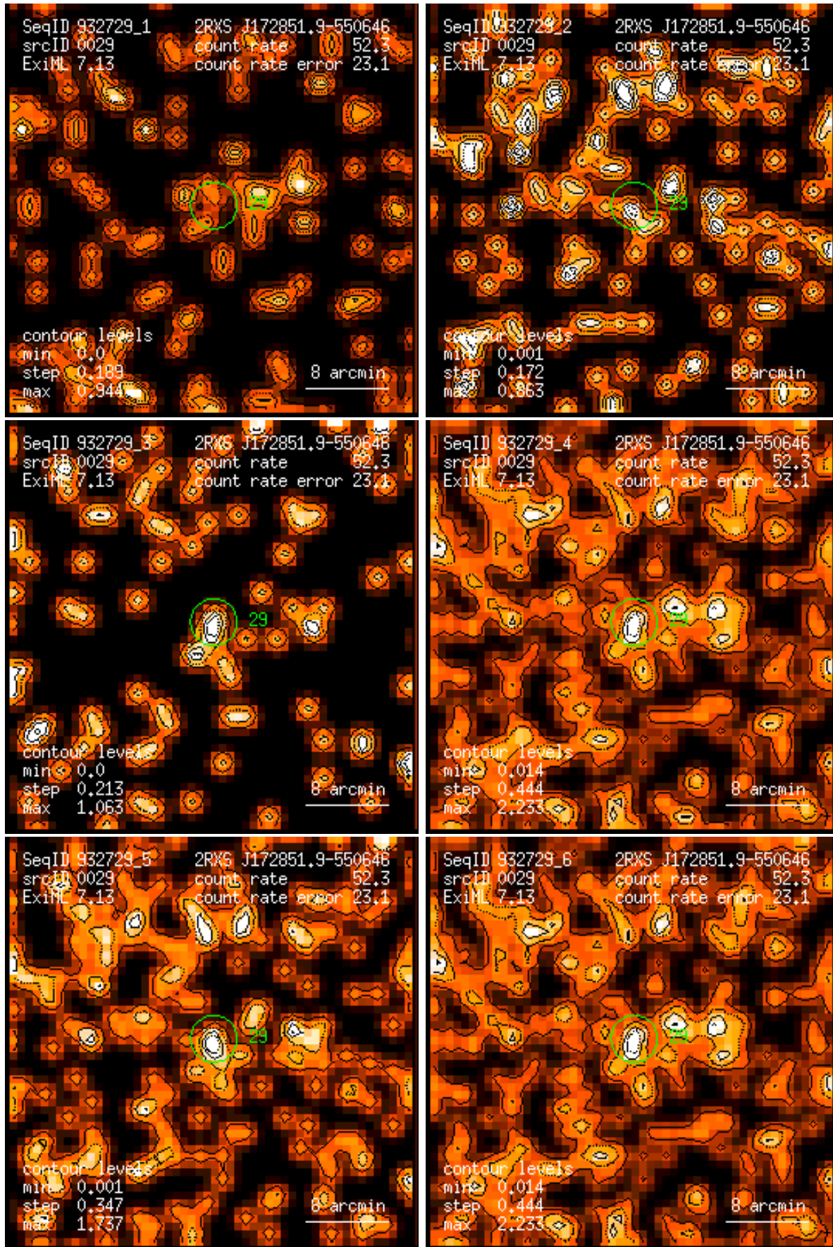
Figure 29: RASS 932729: detection 0029: band rate images, Gaussian filter: (1) PSPC channels 11 – 41, (2) 52 – 90, (3) 91 – 201, (4) 11 – 235, (5) 52 – 201, (6) 11 – 201. Broad band rates in counts/ks. Band rate contour levels in counts/ks/arcmin 2 .
