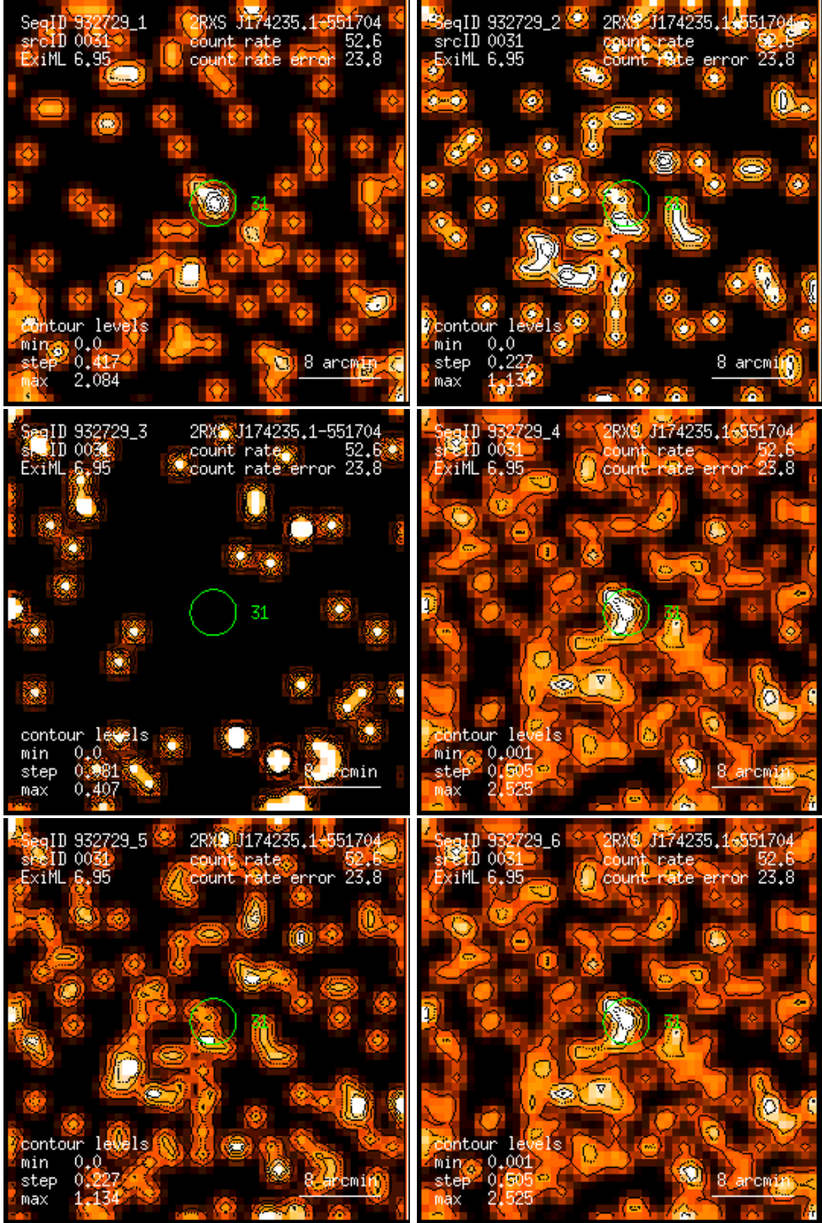
Figure 31: RASS 932729: detection 0031: band rate images, Gaussian filter: (1) PSPC channels 11 – 41, (2) 52 – 90, (3) 91 – 201, (4) 11 – 235, (5) 52 – 201, (6) 11 – 201. Broad band rates in counts/ks. Band rate contour levels in counts/ks/arcmin 2 .
