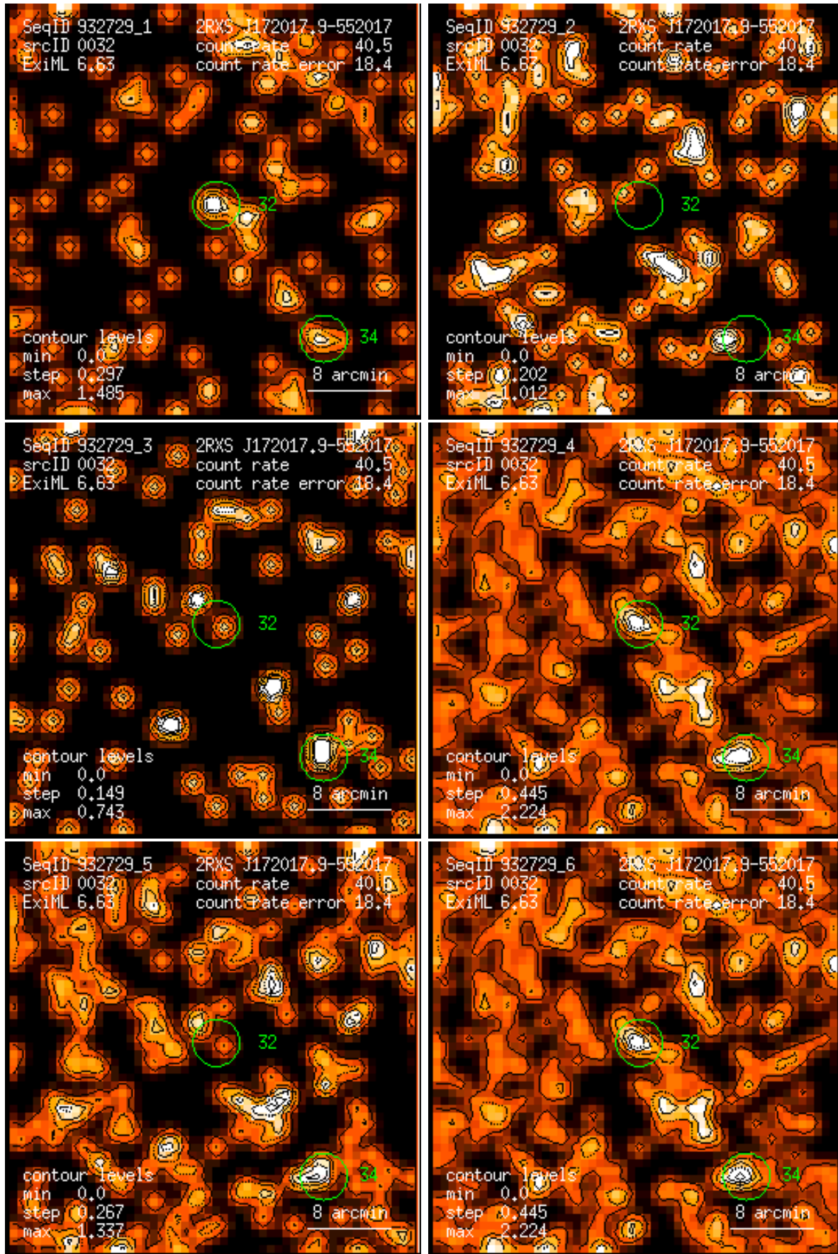
Figure 32: RASS 932729: detection 0032: band rate images, Gaussian filter: (1) PSPC channels 11 – 41, (2) 52 – 90, (3) 91 – 201, (4) 11 – 235, (5) 52 – 201, (6) 11 – 201. Broad band rates in counts/ks. Band rate contour levels in counts/ks/arcmin 2 .
