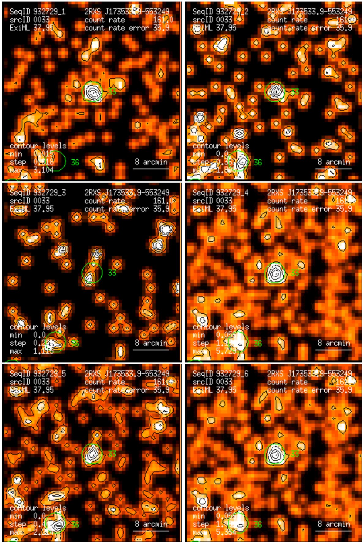
Figure 33: RASS 932729: detection 0033: band rate images, Gaussian filter: (1) PSPC channels 11 – 41, (2) 52 – 90, (3) 91 – 201, (4) 11 – 235, (5) 52 – 201, (6) 11 – 201. Broad band rates in counts/ks. Band rate contour levels in counts/ks/arcmin 2 .
