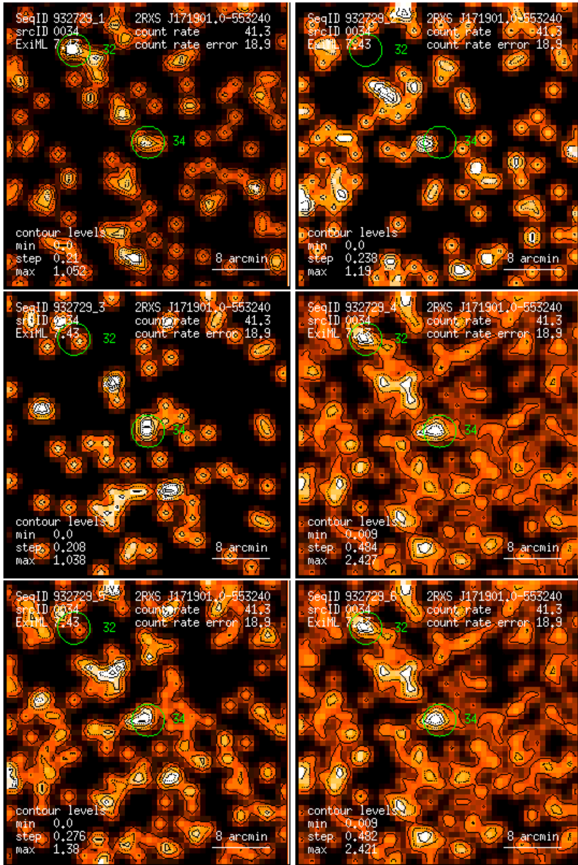
Figure 34: RASS 932729: detection 0034: band rate images, Gaussian filter: (1) PSPC channels 11 – 41, (2) 52 – 90, (3) 91 – 201, (4) 11 – 235, (5) 52 – 201, (6) 11 – 201. Broad band rates in counts/ks. Band rate contour levels in counts/ks/arcmin 2 .
