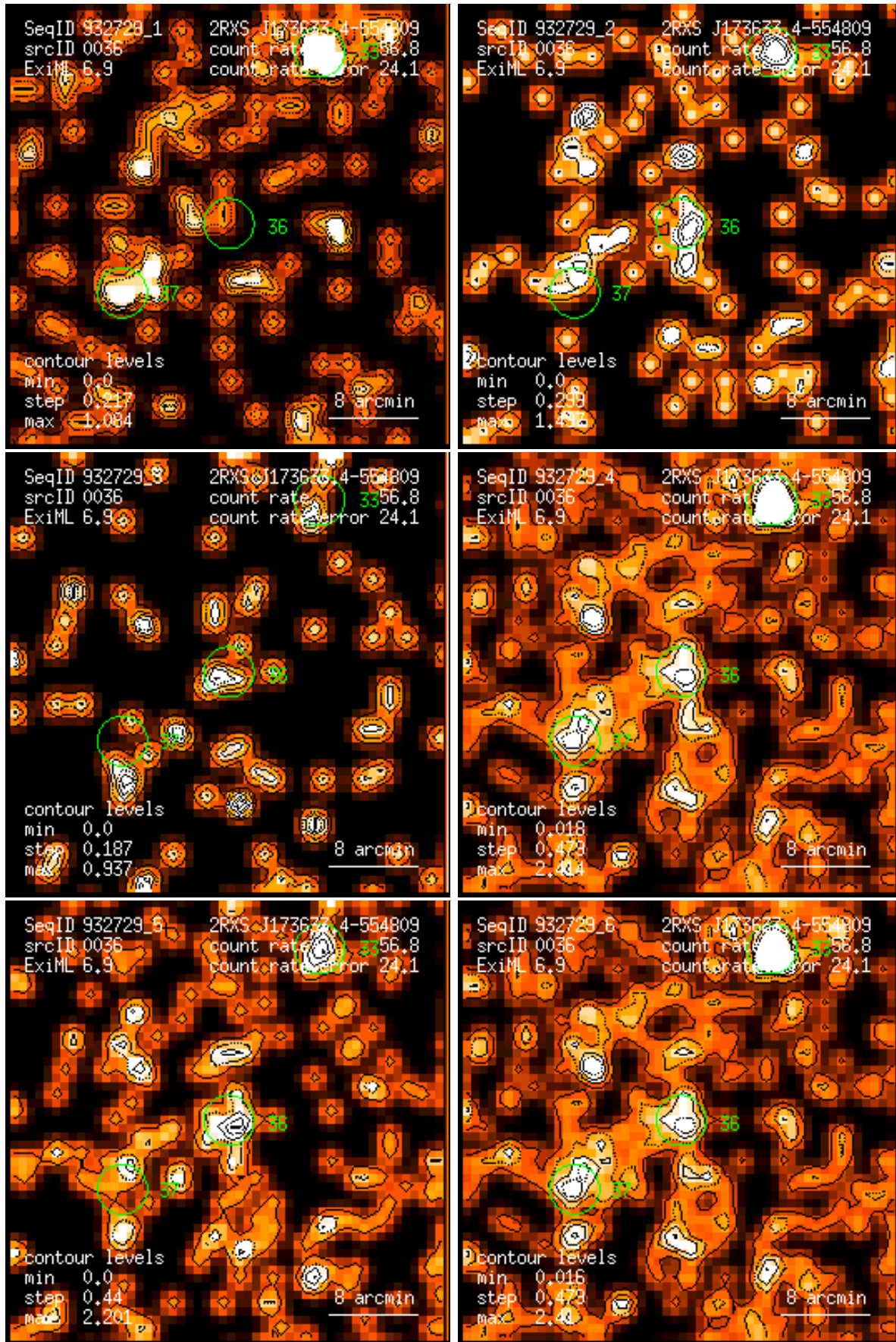
Figure 36: RASS 932729: detection 0036: band rate images, Gaussian filter: (1) PSPC channels 11 – 41, (2) 52 – 90, (3) 91 – 201, (4) 11 – 235, (5) 52 – 201, (6) 11 – 201. Broad band rates in counts/ks. Band rate contour levels in counts/ks/arcmin 2 .
