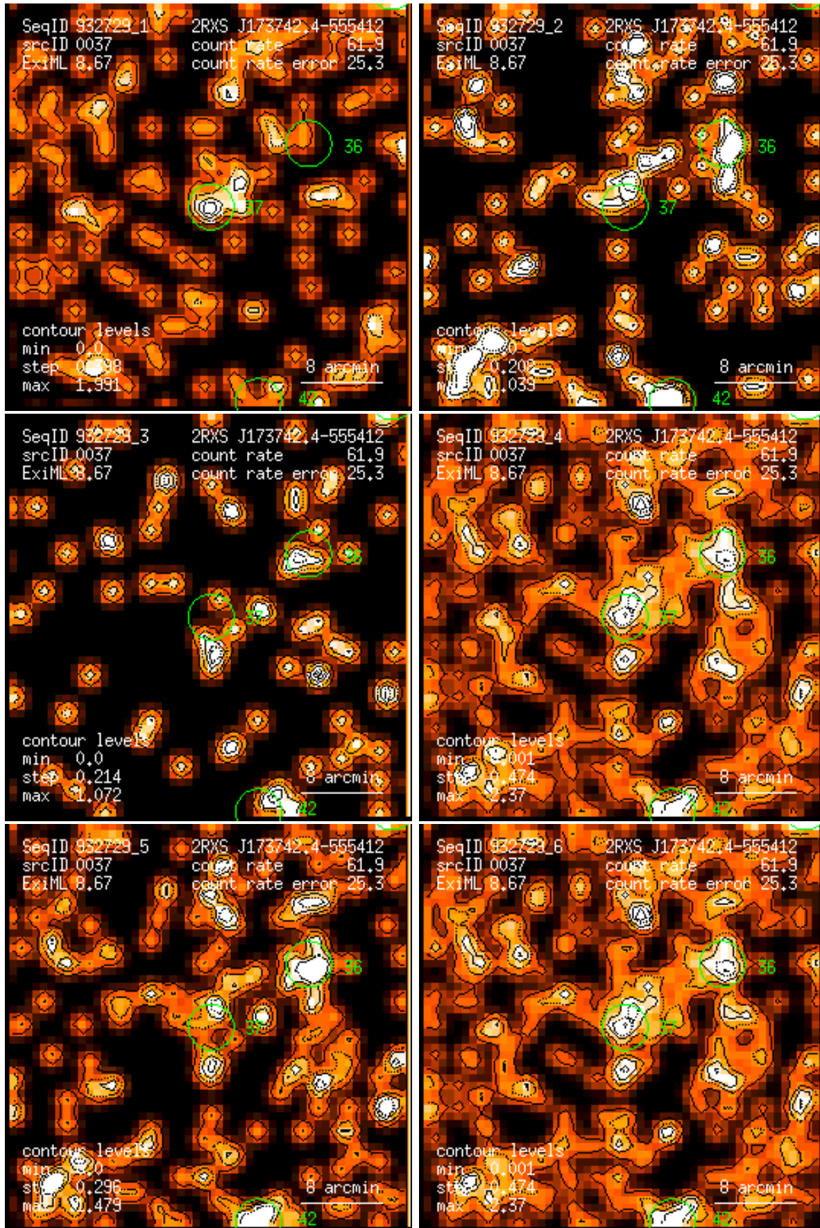
Figure 37: RASS 932729: detection 0037: band rate images, Gaussian filter: (1) PSPC channels 11 – 41, (2) 52 – 90, (3) 91 – 201, (4) 11 – 235, (5) 52 – 201, (6) 11 – 201. Broad band rates in counts/ks. Band rate contour levels in counts/ks/arcmin 2 .
