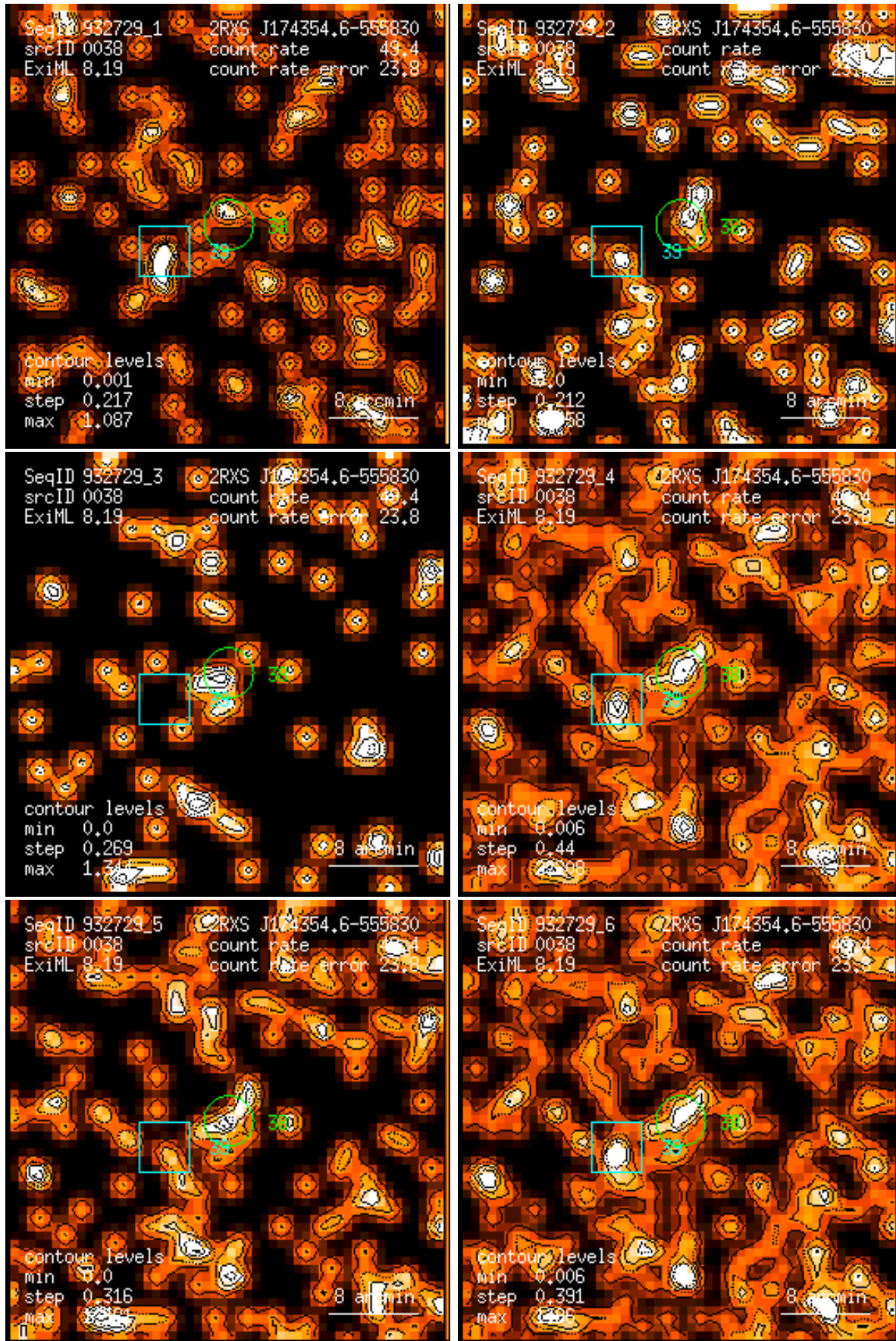
Figure 38: RASS 932729: detection 0038: band rate images, Gaussian filter: (1) PSPC channels 11 – 41, (2) 52 – 90, (3) 91 – 201, (4) 11 – 235, (5) 52 – 201, (6) 11 – 201. Broad band rates in counts/ks. Band rate contour levels in counts/ks/arcmin 2 .
