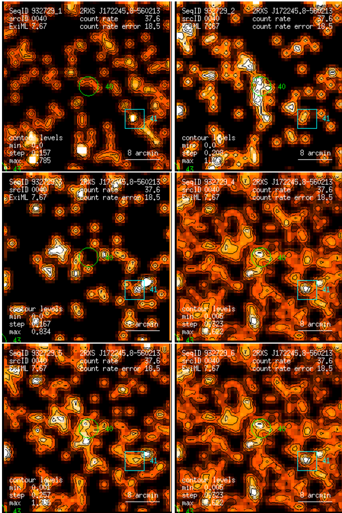
Figure 40: RASS 932729: detection 0040: band rate images, Gaussian filter: (1) PSPC channels 11 – 41, (2) 52 – 90, (3) 91 – 201, (4) 11 – 235, (5) 52 – 201, (6) 11 – 201. Broad band rates in counts/ks. Band rate contour levels in counts/ks/arcmin 2 .
