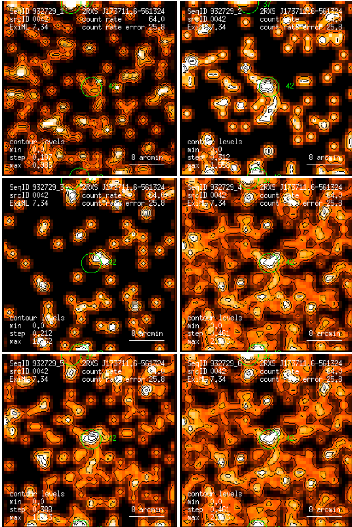
Figure 42: RASS 932729: detection 0042: band rate images, Gaussian filter: (1) PSPC channels 11 – 41, (2) 52 – 90, (3) 91 – 201, (4) 11 – 235, (5) 52 – 201, (6) 11 – 201. Broad band rates in counts/ks. Band rate contour levels in counts/ks/arcmin 2 .
