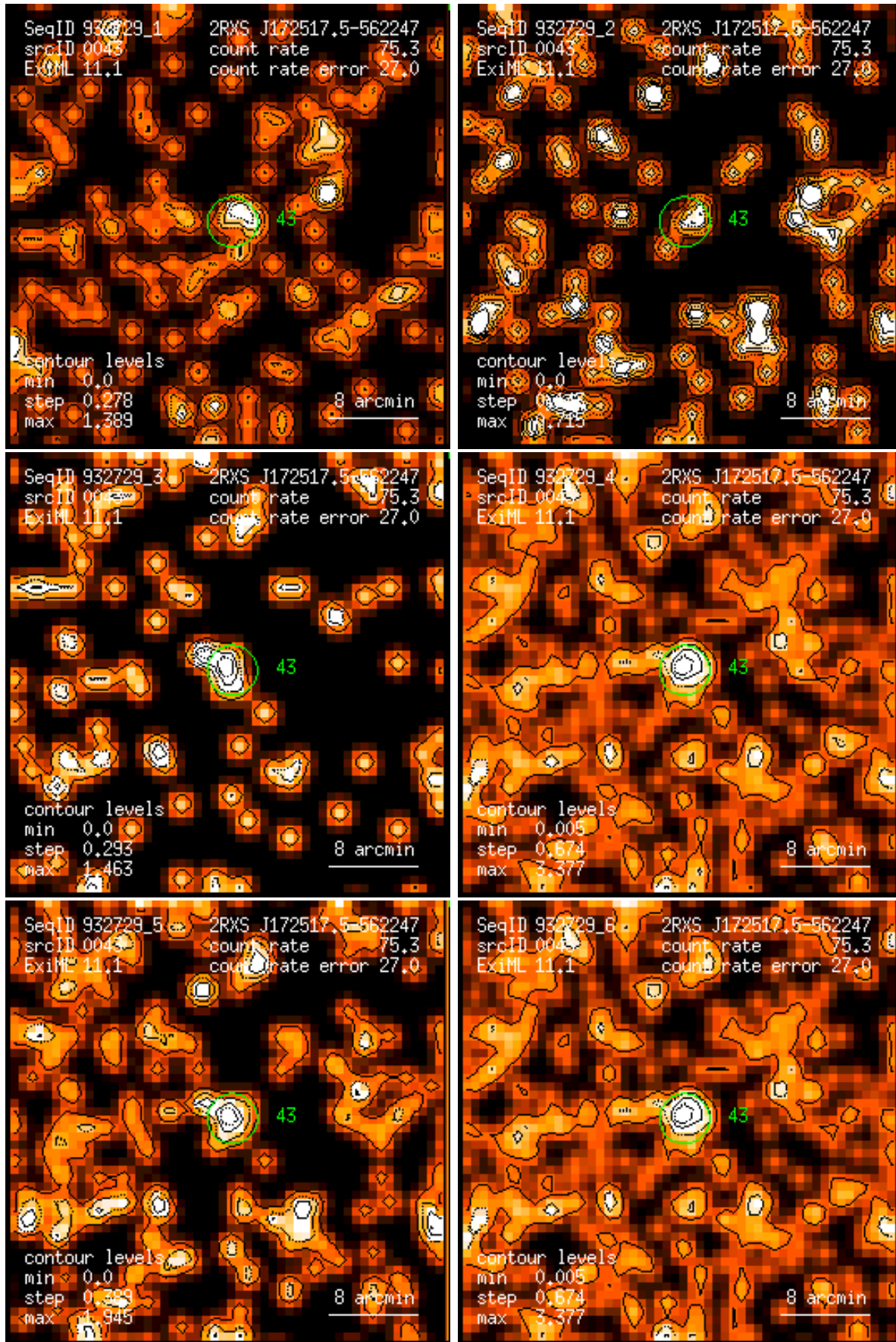
Figure 43: RASS 932729: detection 0043: band rate images, Gaussian filter: (1) PSPC channels 11 – 41, (2) 52 – 90, (3) 91 – 201, (4) 11 – 235, (5) 52 – 201, (6) 11 – 201. Broad band rates in counts/ks. Band rate contour levels in counts/ks/arcmin 2 .
