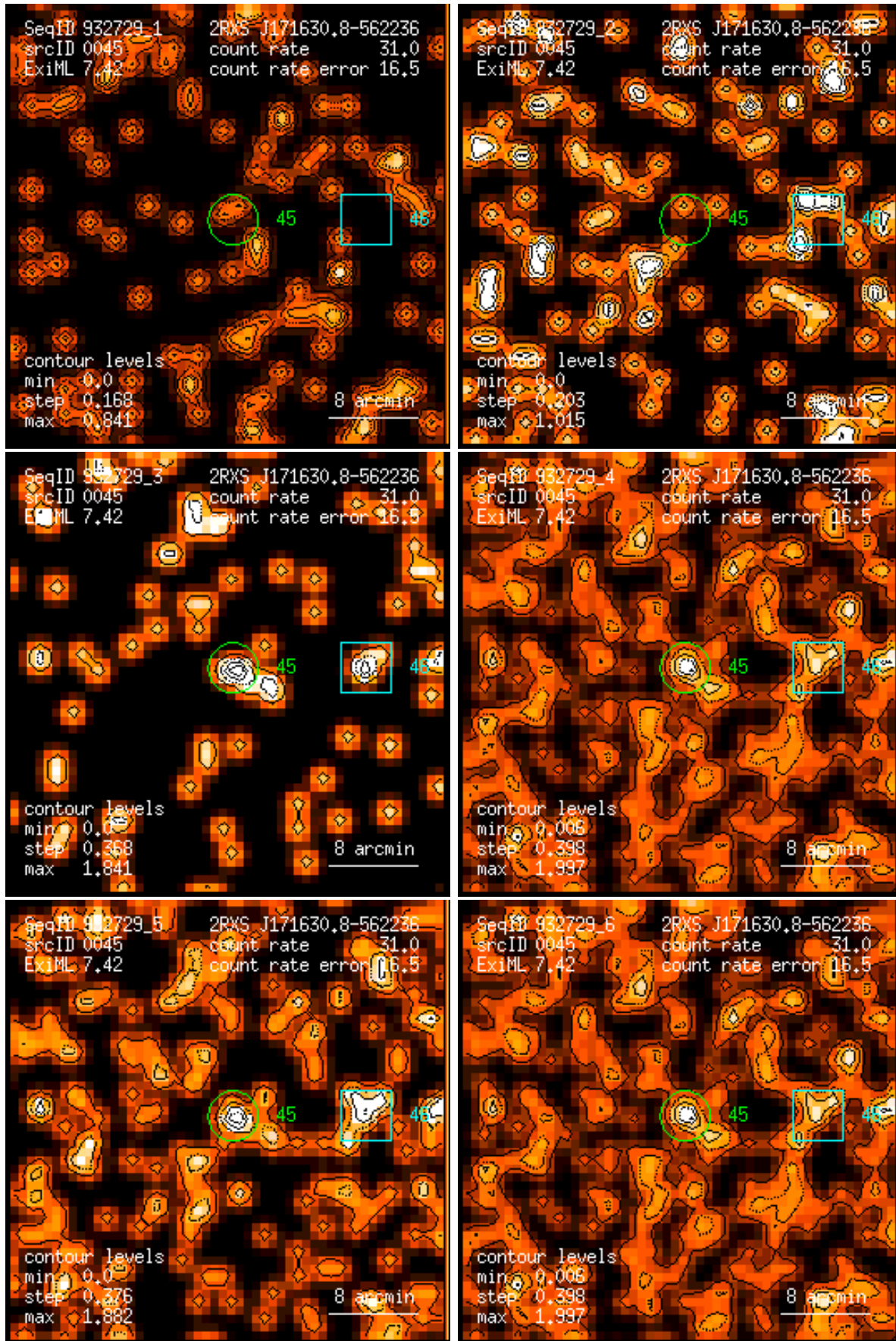
Figure 45: RASS 932729: detection 0045: band rate images, Gaussian filter: (1) PSPC channels 11 – 41, (2) 52 – 90, (3) 91 – 201, (4) 11 – 235, (5) 52 – 201, (6) 11 – 201. Broad band rates in counts/ks. Band rate contour levels in counts/ks/arcmin 2 .
