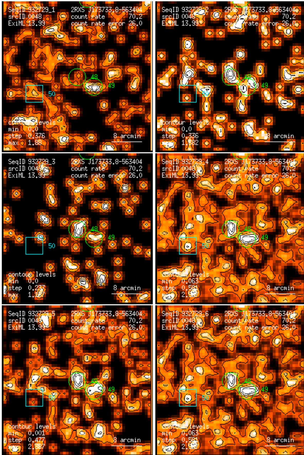
Figure 48: RASS 932729: detection 0048: band rate images, Gaussian filter: (1) PSPC channels 11 – 41, (2) 52 – 90, (3) 91 – 201, (4) 11 – 235, (5) 52 – 201, (6) 11 – 201. Broad band rates in counts/ks. Band rate contour levels in counts/ks/arcmin 2 .
