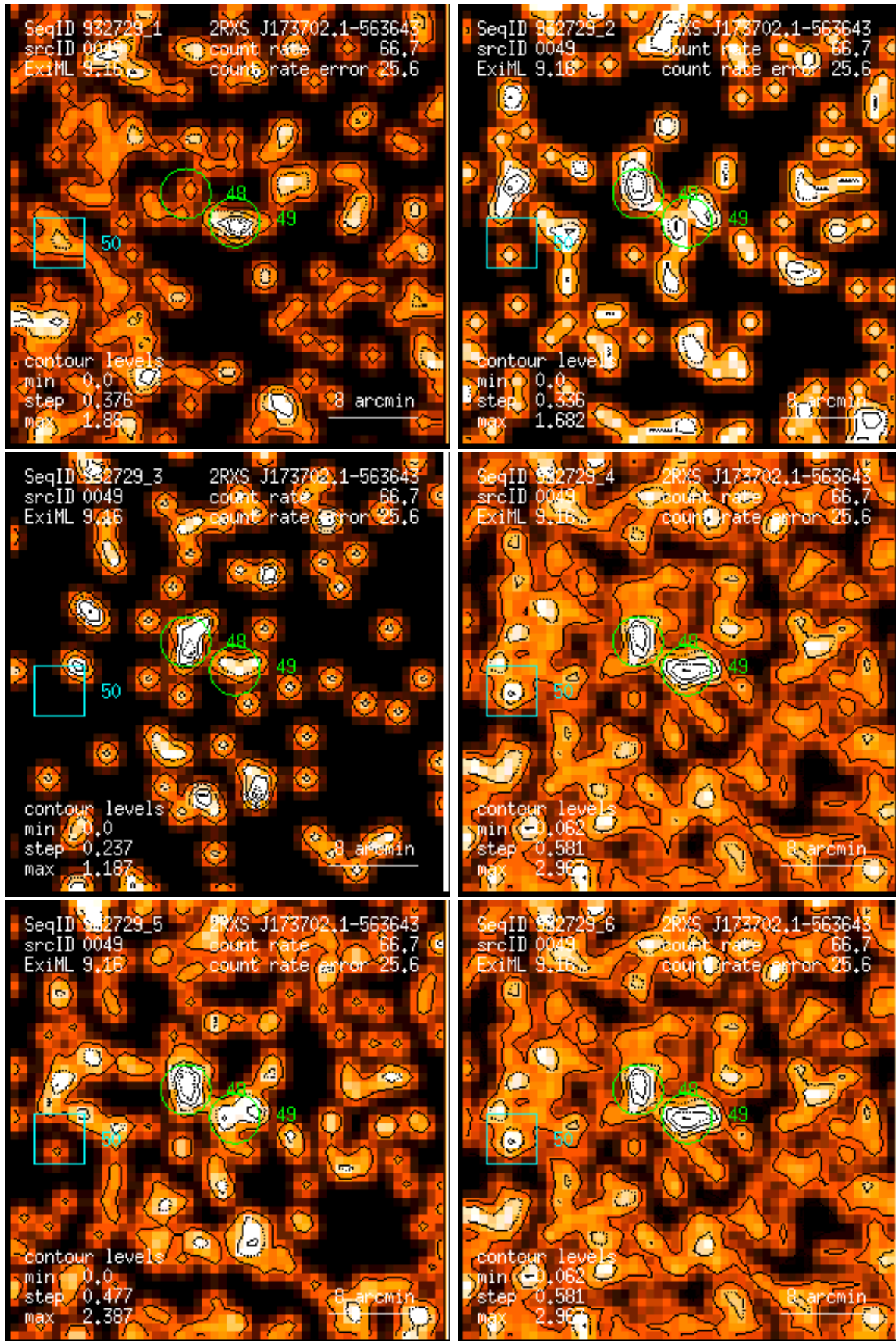
Figure 49: RASS 932729: detection 0049: band rate images, Gaussian filter: (1) PSPC channels 11 – 41, (2) 52 – 90, (3) 91 – 201, (4) 11 – 235, (5) 52 – 201, (6) 11 – 201. Broad band rates in counts/ks. Band rate contour levels in counts/ks/arcmin 2 .
