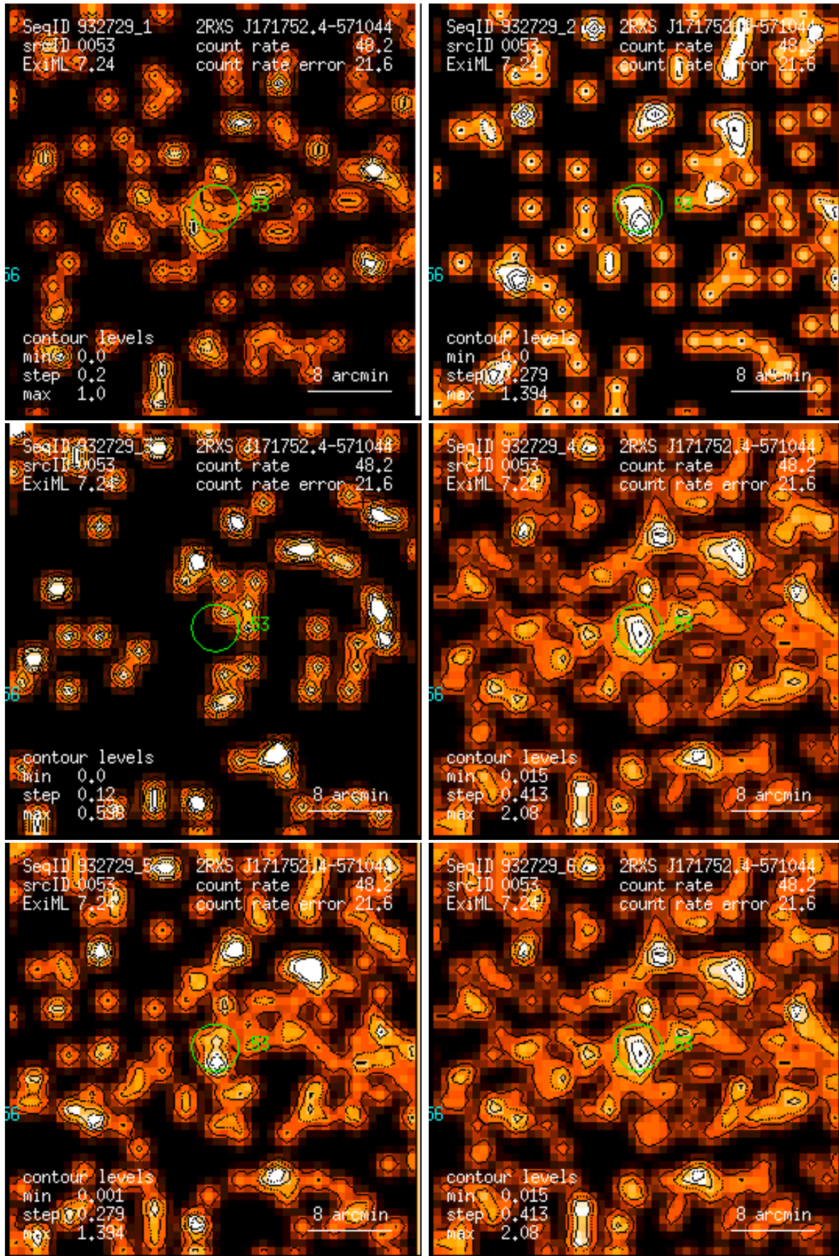
Figure 53: RASS 932729: detection 0053: band rate images, Gaussian filter: (1) PSPC channels 11 – 41, (2) 52 – 90, (3) 91 – 201, (4) 11 – 235, (5) 52 – 201, (6) 11 – 201. Broad band rates in counts/ks. Band rate contour levels in counts/ks/arcmin 2 .
