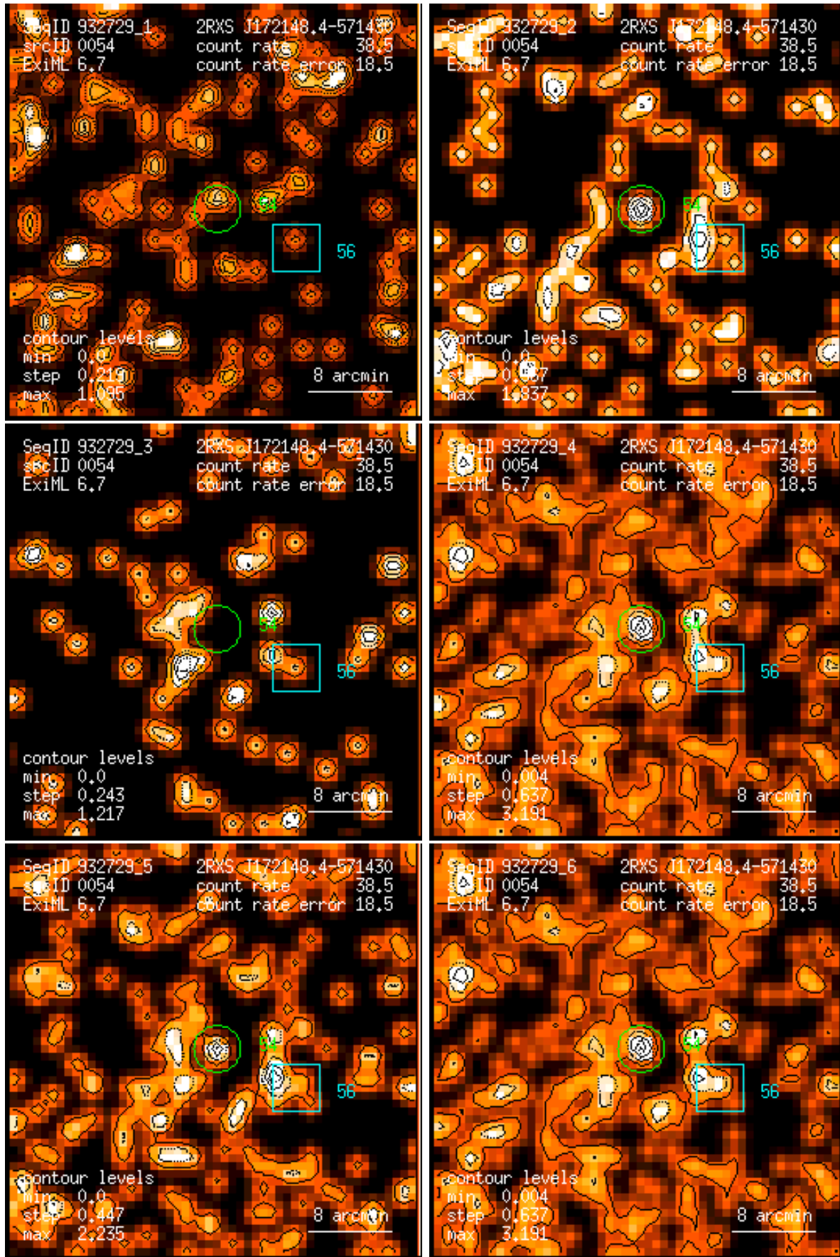
Figure 54: RASS 932729: detection 0054: band rate images, Gaussian filter: (1) PSPC channels 11 – 41, (2) 52 – 90, (3) 91 – 201, (4) 11 – 235, (5) 52 – 201, (6) 11 – 201. Broad band rates in counts/ks. Band rate contour levels in counts/ks/arcmin 2 .
