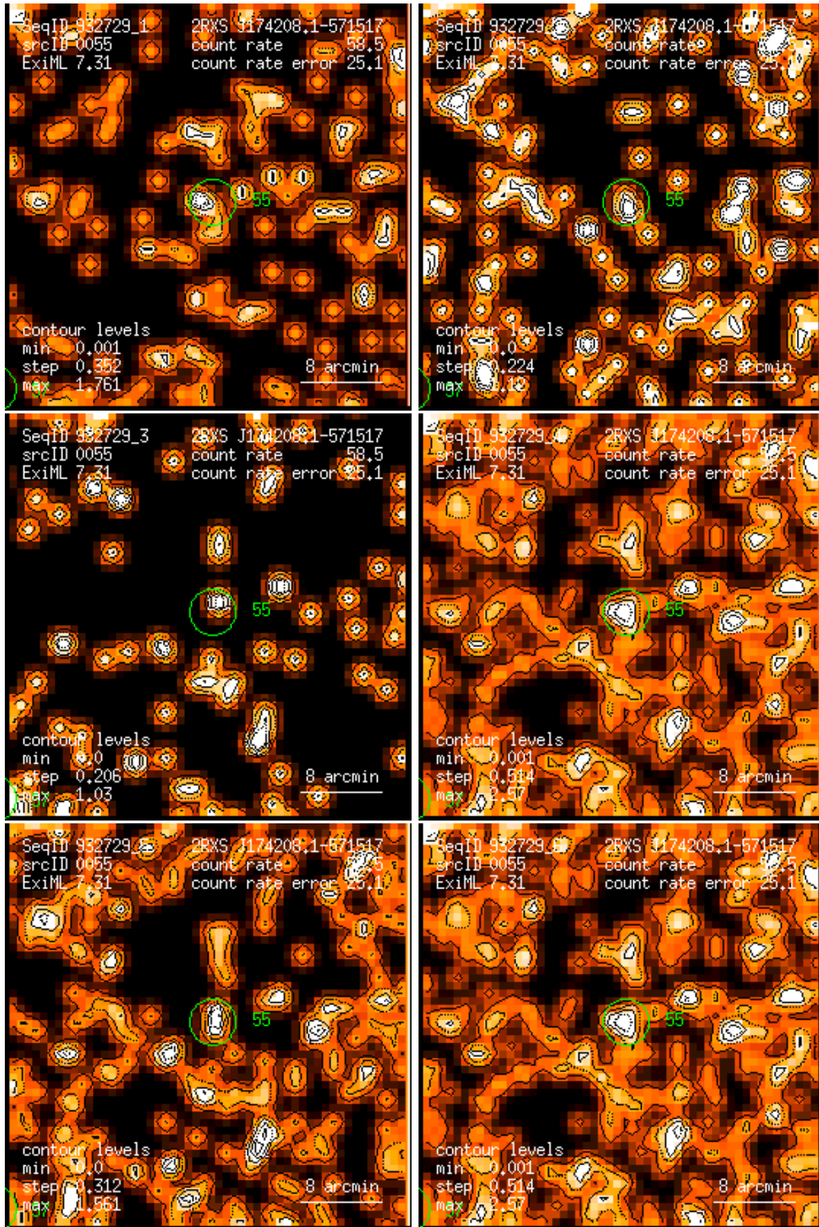
Figure 55: RASS 932729: detection 0055: band rate images, Gaussian filter: (1) PSPC channels 11 – 41, (2) 52 – 90, (3) 91 – 201, (4) 11 – 235, (5) 52 – 201, (6) 11 – 201. Broad band rates in counts/ks. Band rate contour levels in counts/ks/arcmin 2 .
